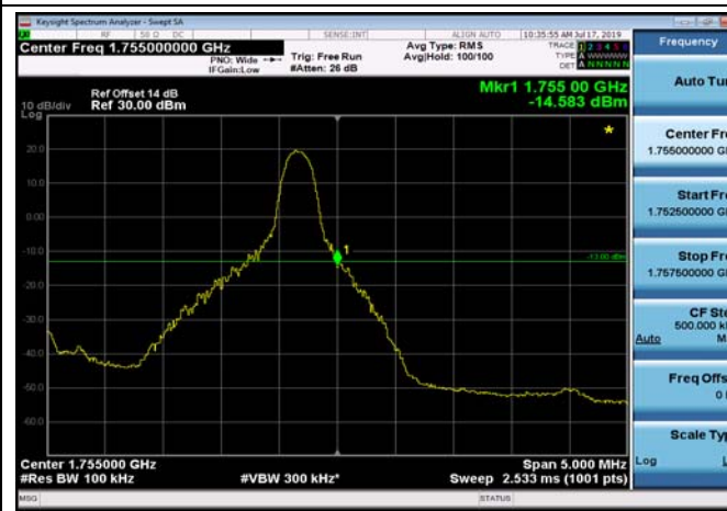
HighRange_FDD04_5MHz_1752.5_OneRB _high_QPSK
