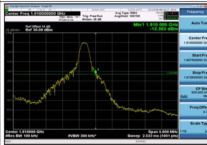
HighRange_FDD02_5MHz_1907.5_OneRB _high_Q16
