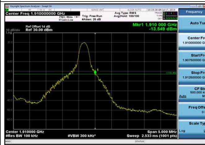
HighRange_FDD02_5MHz_1907.5_OneRB _high_QPSK
