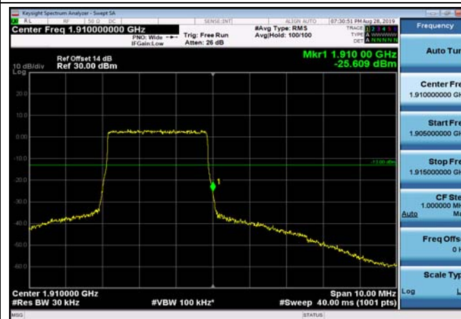
HighRange_FDD02_5MHz_1907.5_OneRB _high_Q16
