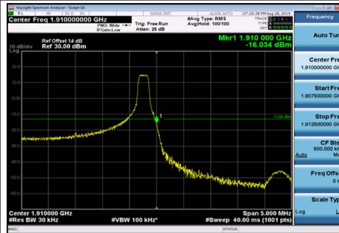
HighRange_FDD02_3MHz_1908.5_fullIRB _High_Q16
