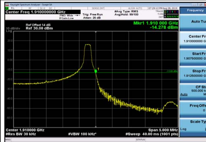
HighRange_FDD02_3MHz_1908.5_fullIRB _High_QPSK
