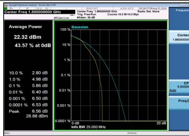
FDD02_HighRange_20MHz_1900_OneRB _high_Q16
