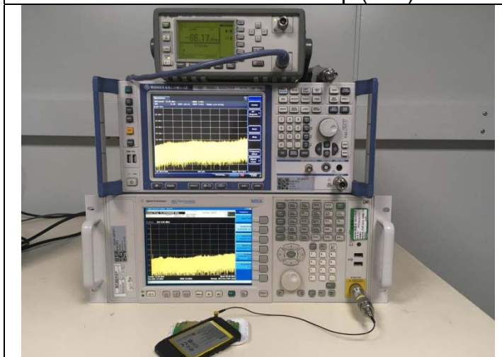
RF Conducted Test setup (WIFI)
