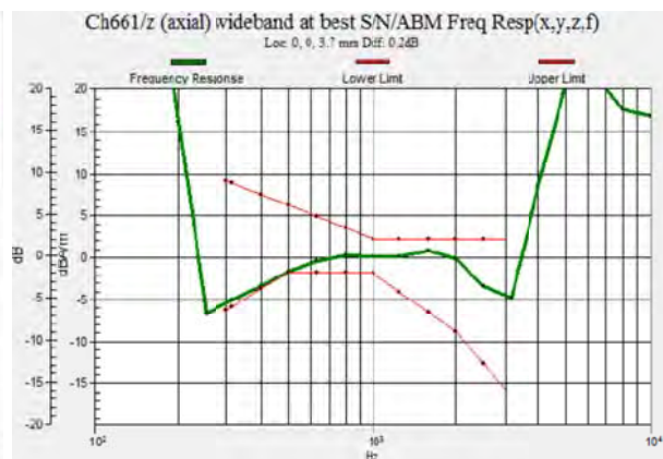
Fig 7.7 GSM1900 Ch661
