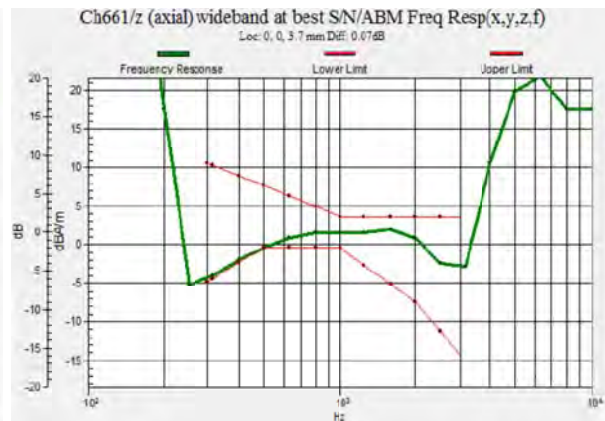
Fig 7.2 GSM1900 Ch661
