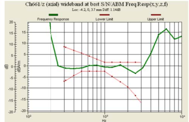
Fig 7.2 GSM1900 Ch661
