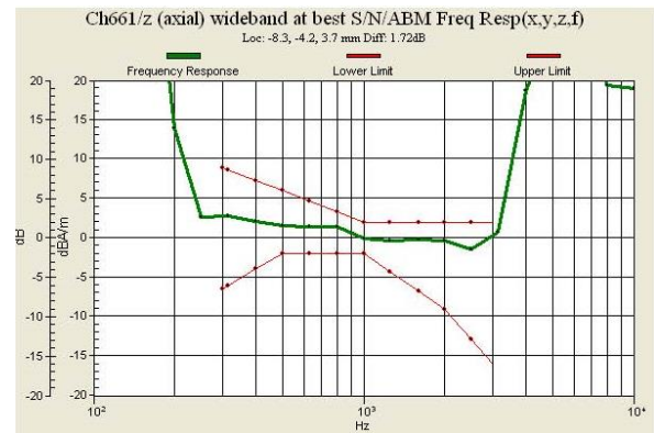
Fig 7.2 GSM1900 Ch661
