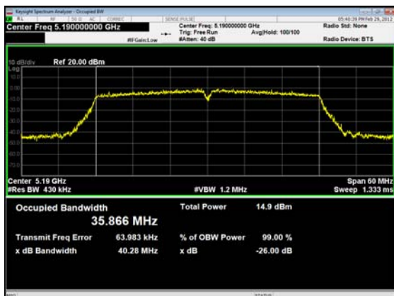
U-NII-1, 802.11ac VHT40 Carrier frequency (MHz): 5190
