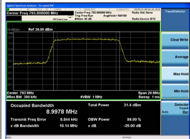
LTE Band 14 QPSK 10MHz CH-Middle
