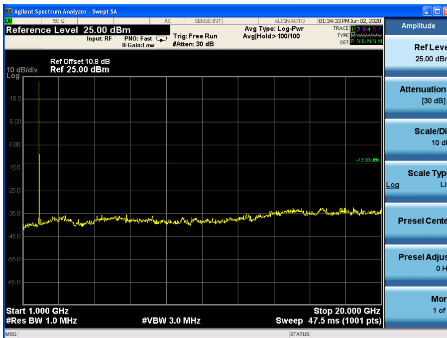
Channel 9400, 1GHz~20GHz
