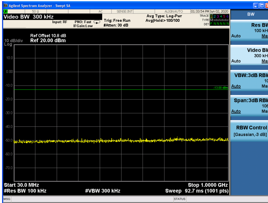
Channel 9400, 30MHz~1GHz
