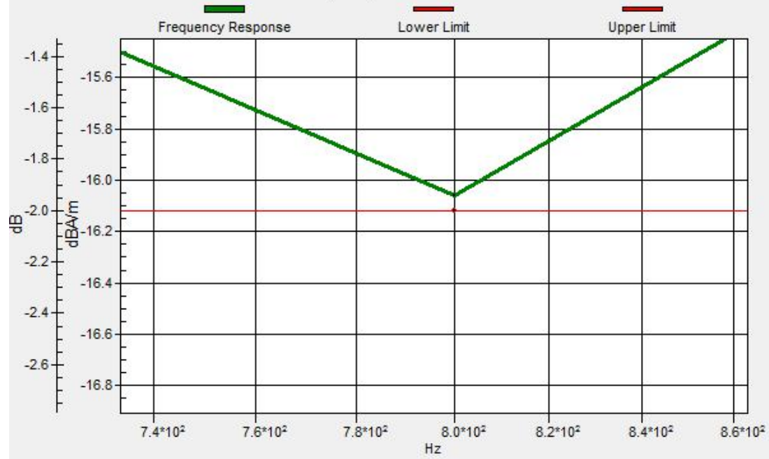
General Scans_LTE band4_T-Coil_HAC 2 2 2/z (axial) wideband at best S/N/ABM Freq Resp(x,y,z,f) Loc: 3.6, -12.4, 3.7 mm Diff: 0.06dB
