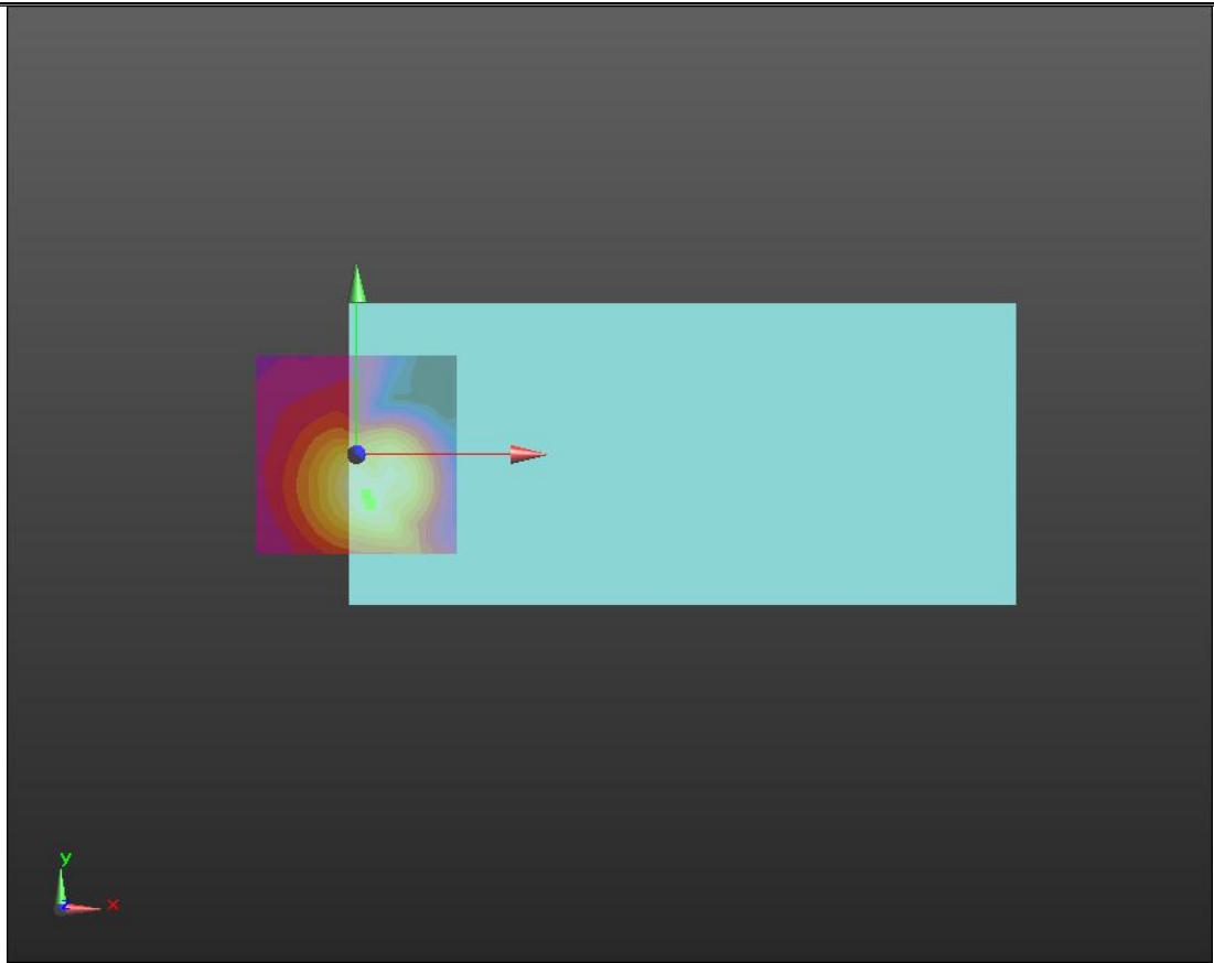
General Scans_LTE band4_T-Coil_HAC 2 2 2/z (axial) wideband at best S/N/ABM Freq Resp(x,y,z,f) Loc: 3.6, -12.4, 3.7 mm Diff: 0.06dB
