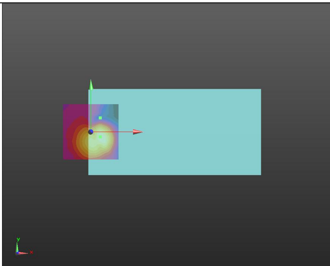
General Scans_WIFI5G UNII-1 802.11a T-Coil_HAC 4/z (axial) wideband at best S/N/ABM Freq Resp(x,y,z,f) Loc: 8.5, 12.5, 3.7 mm Diff: 1.01dB
