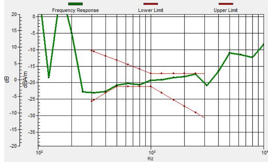
General Scans_LTE band5_T-Coil_HAC 3/z (axial) wideband at best S/N/ABM Freq Resp(x,y,z,f) Loc: 3.7, -12.3, 3.7 mm Diff: 0.18dB
