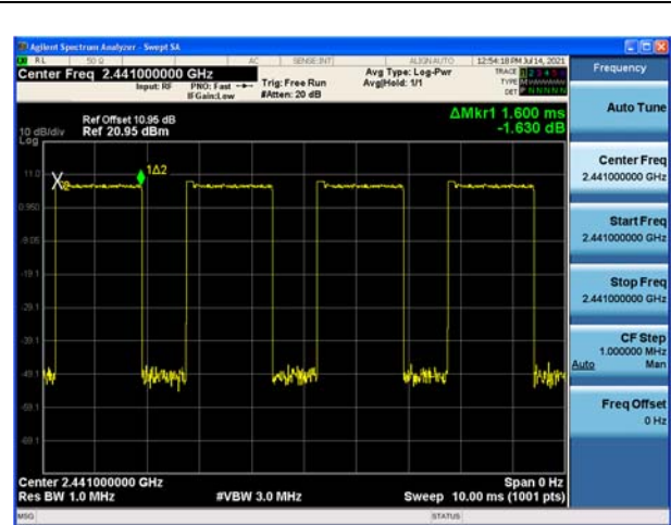
Modulation: π4DQPSK 2DH3 2441MHz
