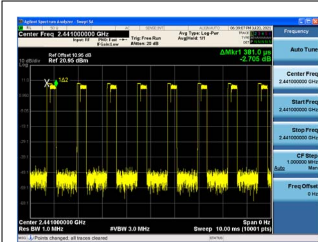
Modulation: π4DQPSK 2DH1 2441MHz
