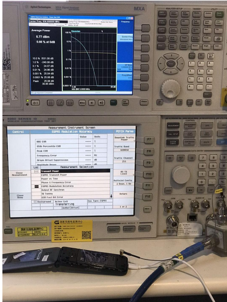
RF Conducted Test setup
