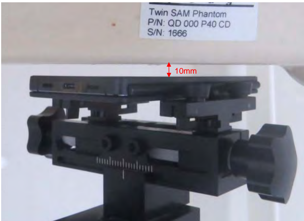
Picture 19: Front Side, the distance from handset to the bottom of the Phantom is 10mm For Single Screen Mode
