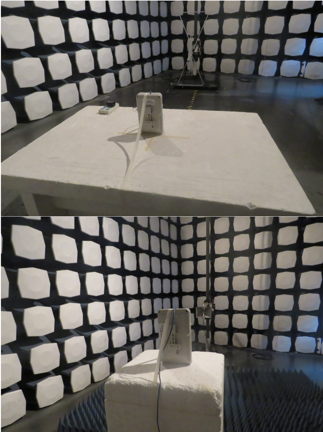
Radiated Spurious Emissions Test setup
