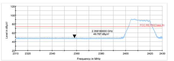
802.11g-Channel 1 Peak
