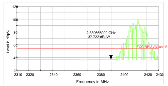
802.11b-Channel 1 Average
