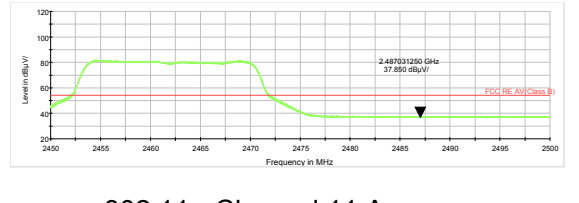
802.11g-Channel 11 Average
