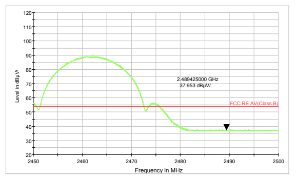
802.11b-Channel 11 Average
