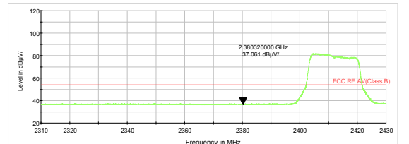
802.11g-Channel 1 Average
