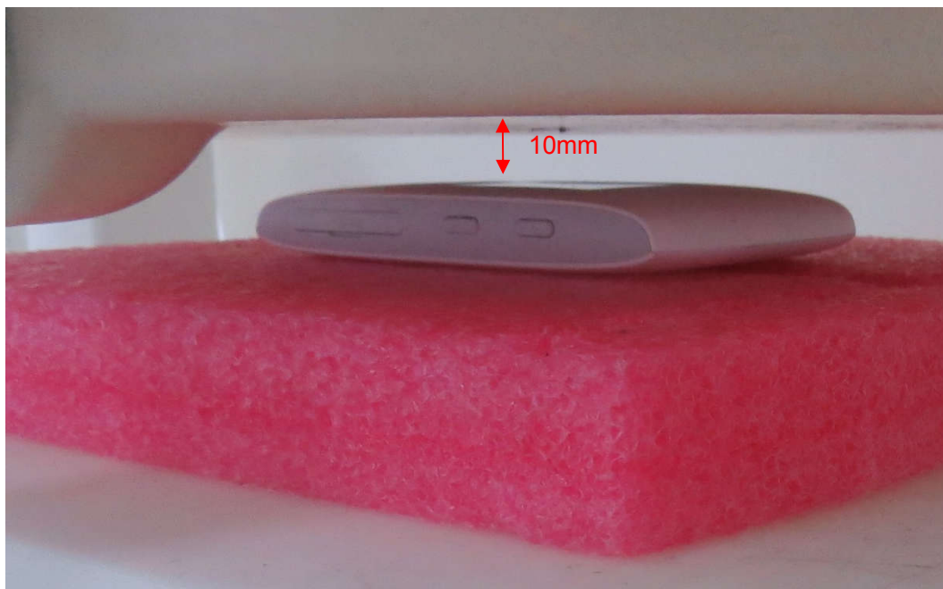
Picture 2: Front Side, the distance from handset to the bottom of the Phantom is 10mm
