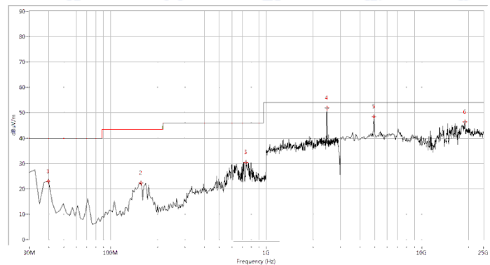
(Antenna Horizontal, 30MHz to 25GHz)
