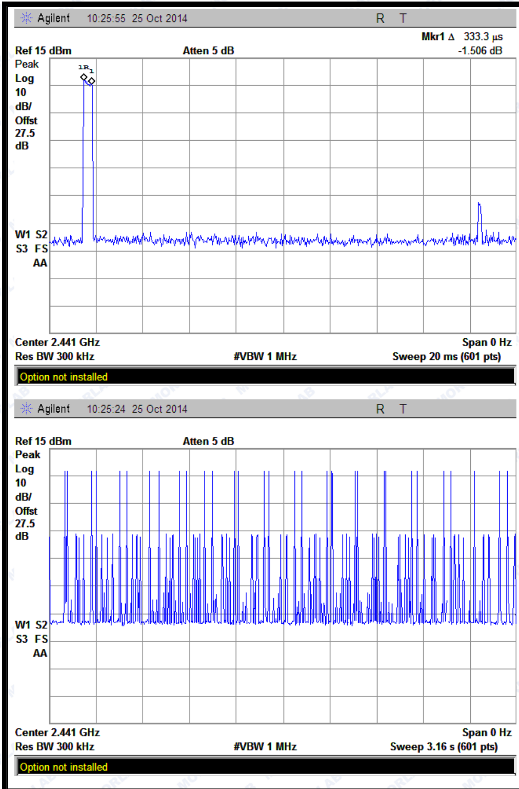
(Plot D: DH1 @ π/4-DQPSK)
