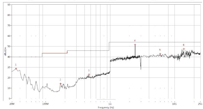
(30MHz to 25GHz, Antenna Horizontal @ GFSK, channel 39)
