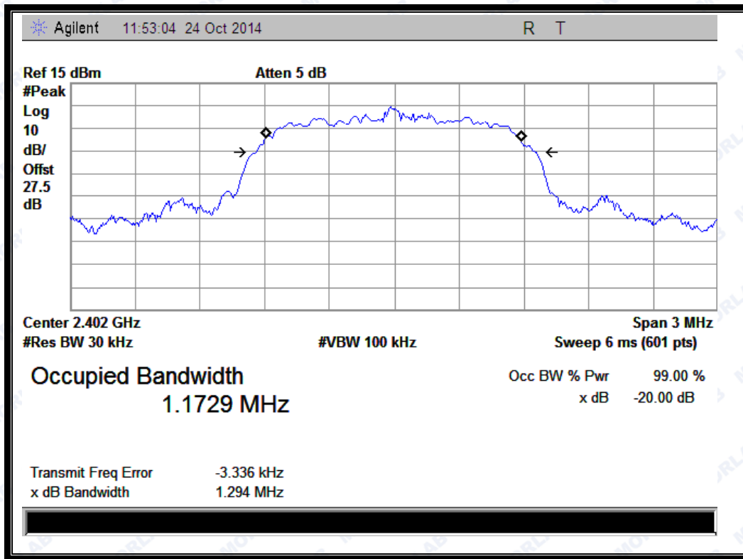
(Plot D: Channel = 2402 @ □/4-DQPSK)
