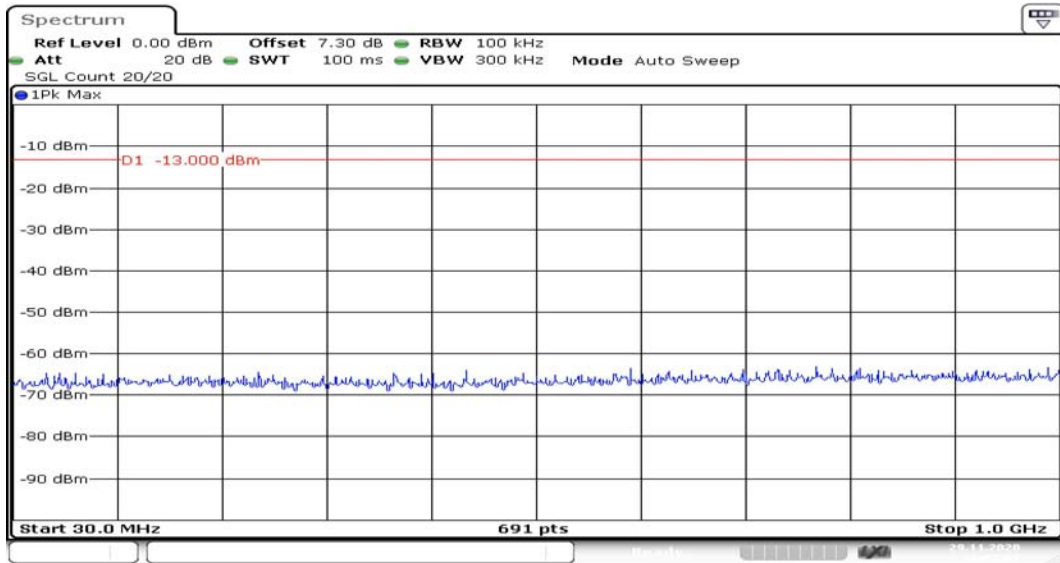
Channel 9400 30MHz~1GHz
