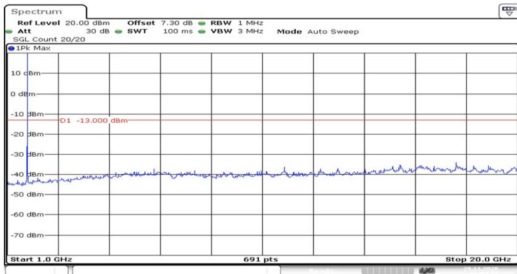
Channel 1412 1GHz~20GHz
