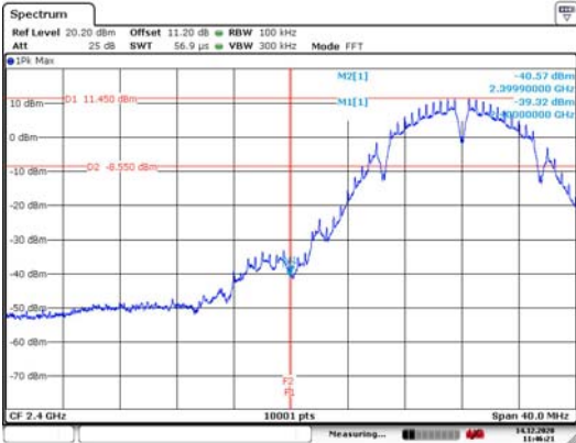
Test Mode: 802.11b Chain1 CH1
