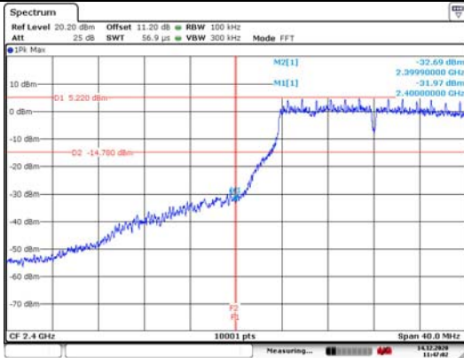
Test Mode: 802.11g Chain1 CH1
