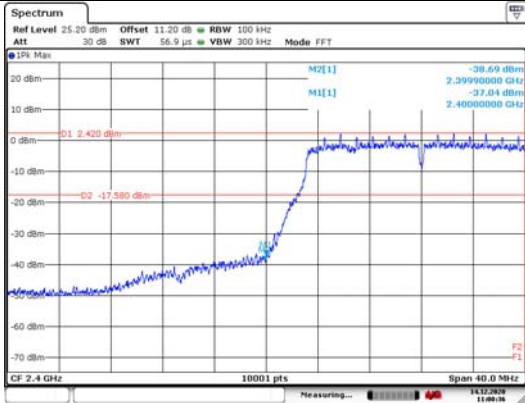
Test Mode: 802.11n HT20 Chain1 CH1
