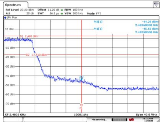
Test Mode: 802.11n HT20 Chain1 CH11
