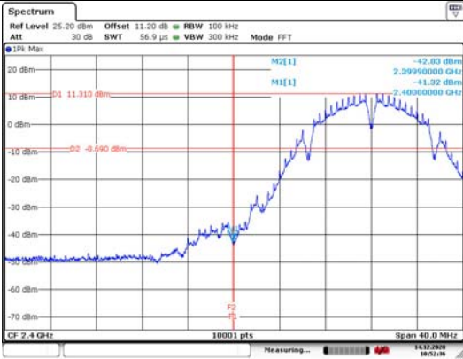
Test Mode: 802.11b Chain1 CH1
