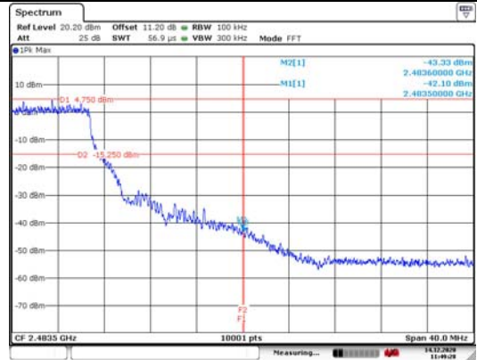
Test Mode: 802.11g Chain1 CH11
