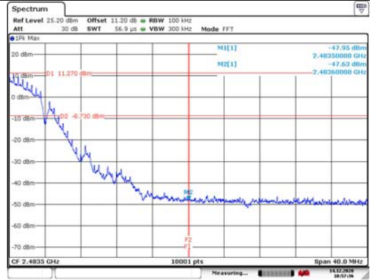
Test Mode: 802.11b Chain1 CH11
