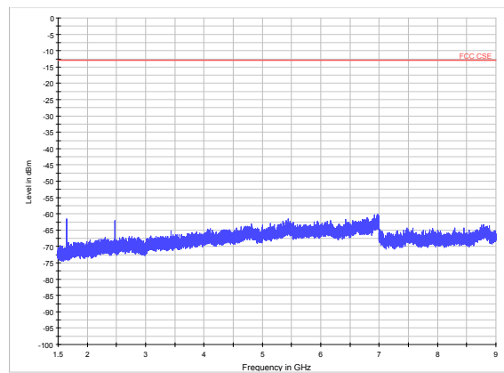
LTE Band 5 1.4MHz CH-Middle 1.5GHz~9GHz
