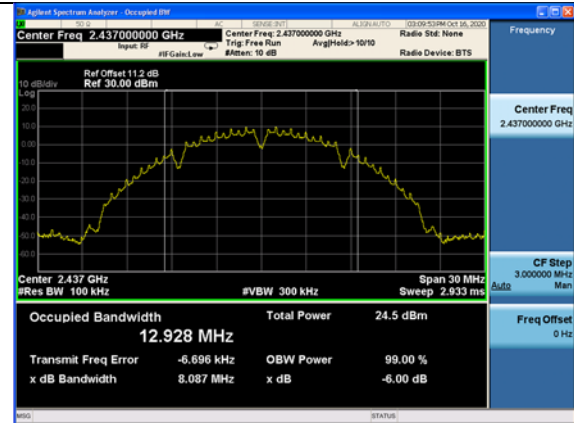
Test Mode: 802.11b Chain1
