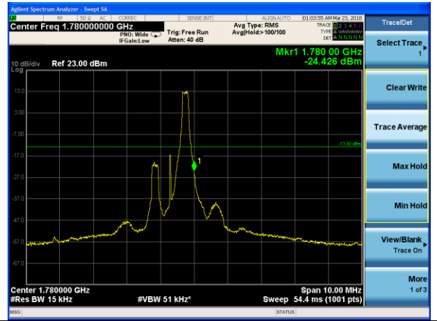
LTE Band 66 16QAM 1.4MHz CH-High, 1 RB
