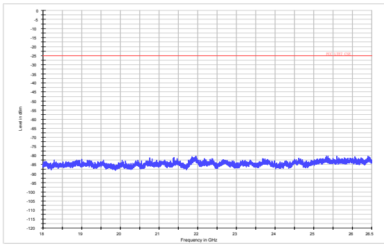
LTE Band 7 20MHz CH-Middle 18GHz~26.5GHz
