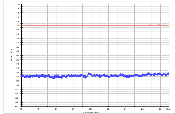
LTE Band 7 10MHz C CH-Low 18GHz~26.5GHz
