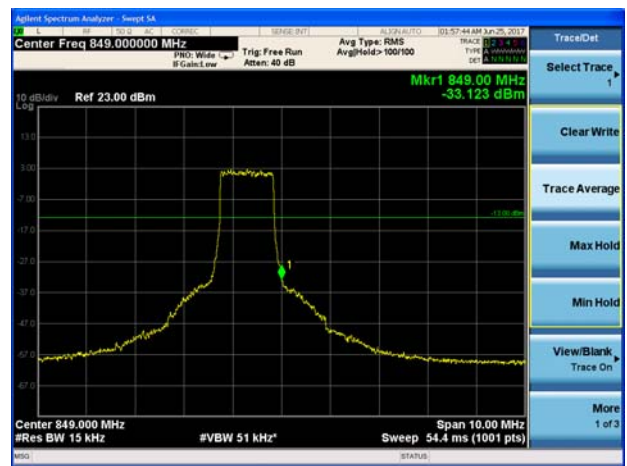
LTE Band 5 16QAM 3MHz CH-High 1RB
