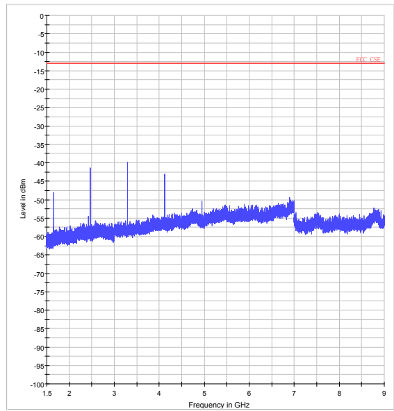
LTE Band 5 1.4MHz CH-Middle 1.5GHz~9GHz
