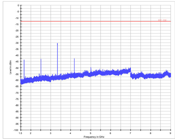
LTE Band 5 3MHz CH-High 1.5GHz~9GHz
