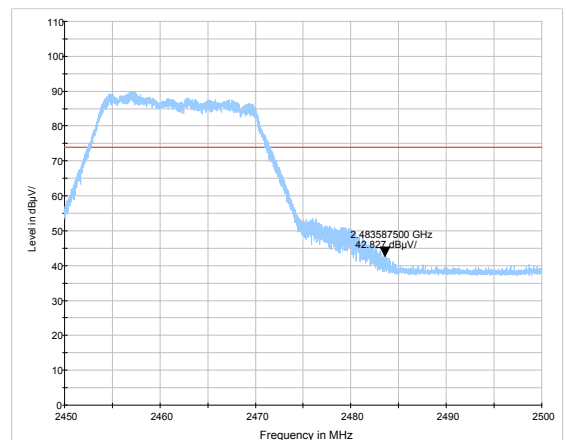
802.11g-Channel 11: Peak
