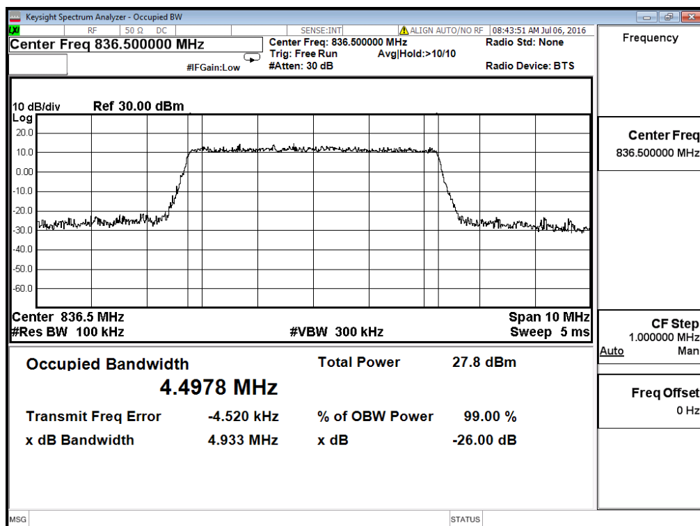
Occupied Bandwidth LTE Band 5/5MHz/16QAM
