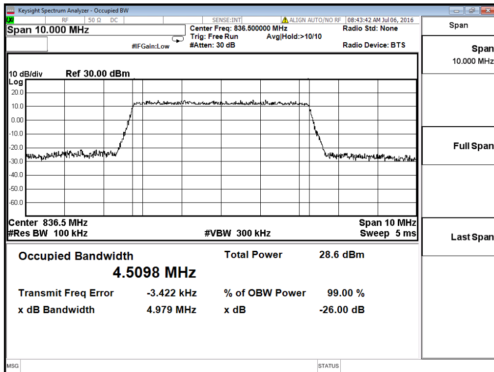
Occupied Bandwidth LTE Band 5/5MHz/QPSK
