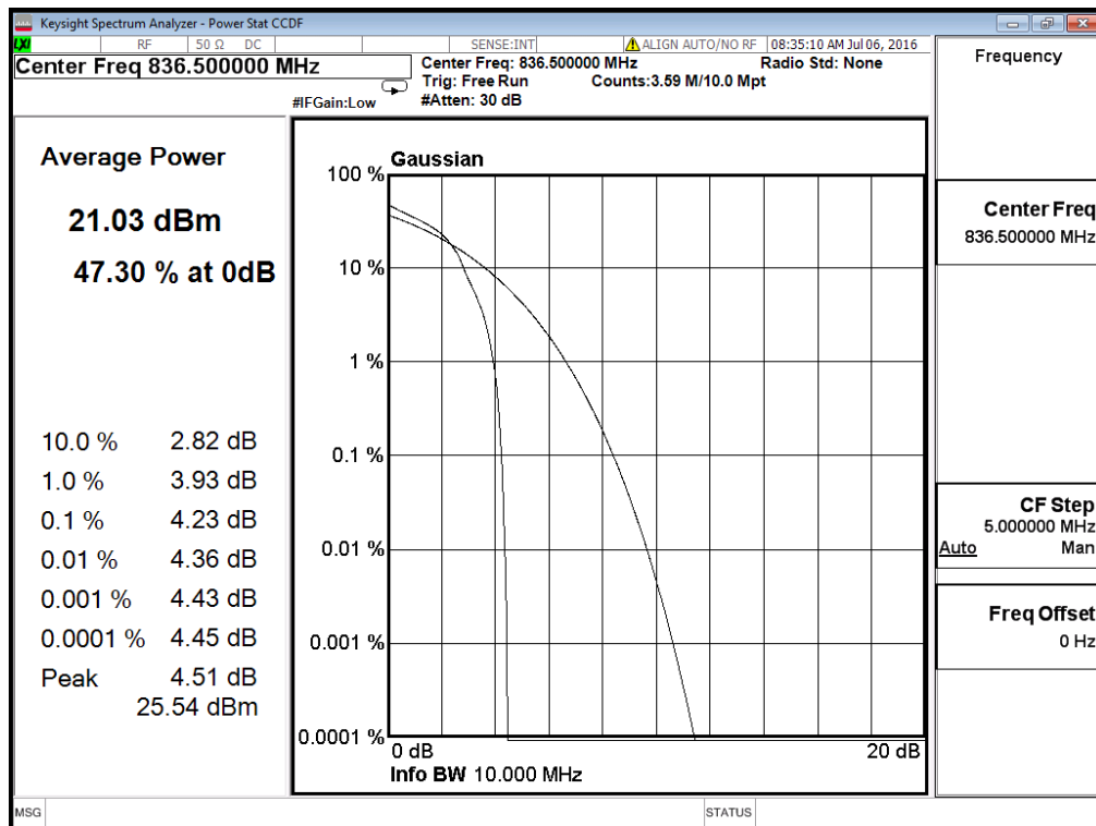
(Plot C3: Band 5/10MHz/16QAM in M Ch 1RB Size)
