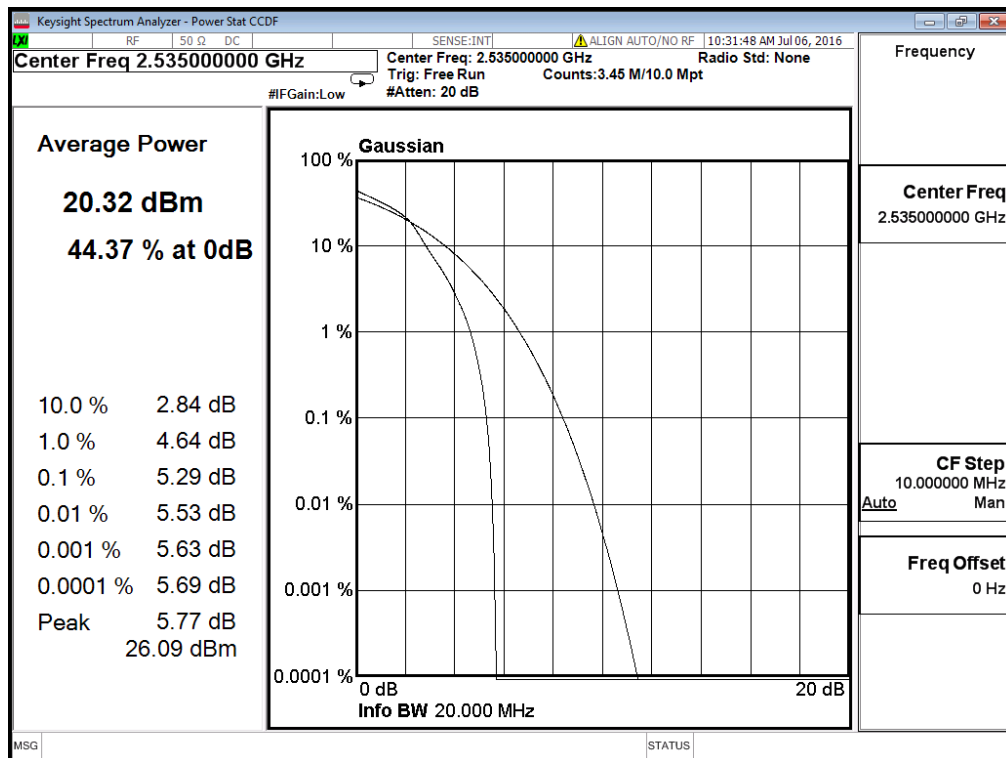
(Plot D3: Band 7/20MHz/16QAM in M Ch 1RB Size)
