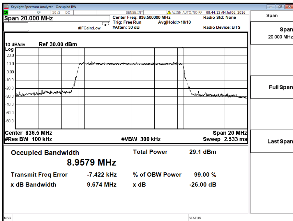
Occupied Bandwidth LTE Band 5/10MHz/QPSK
