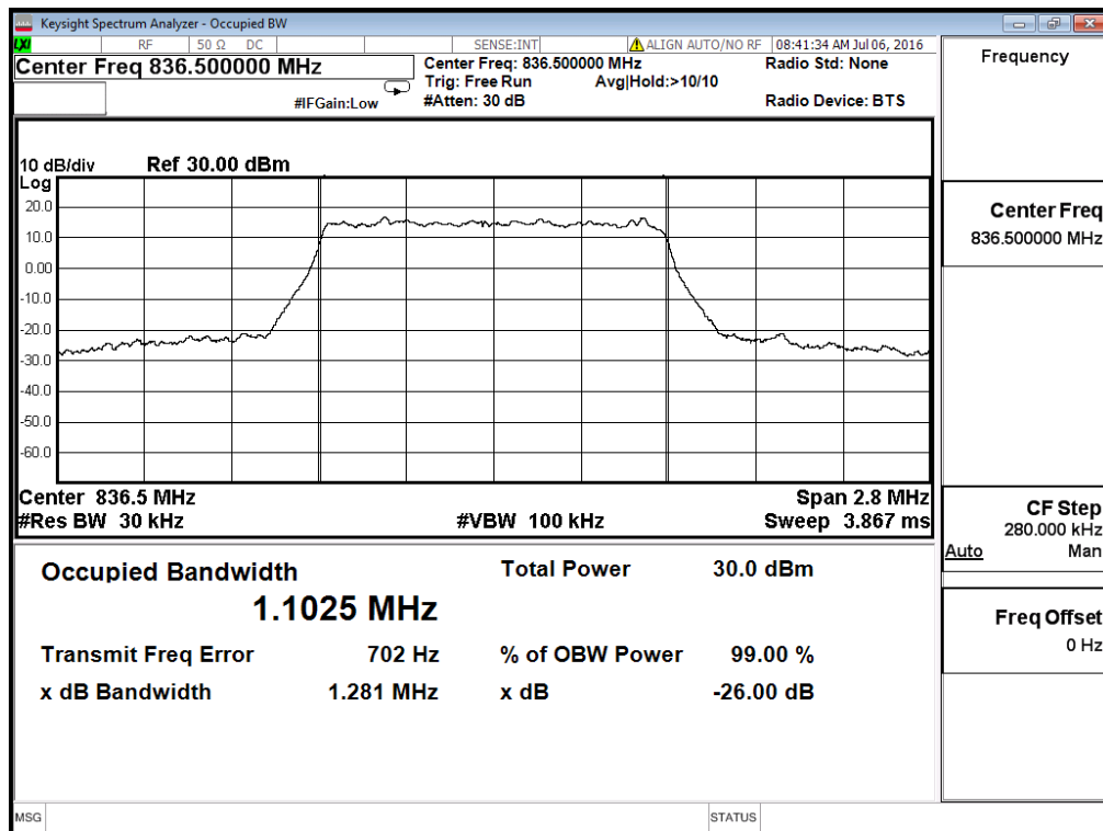
Occupied Bandwidth LTE Band 5/1.4MHz/QPSK
