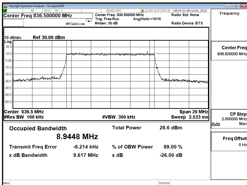
Occupied Bandwidth LTE Band 5/10MHz/16QAM
