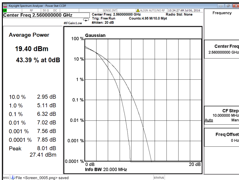
(Plot D6: Band 7/20MHz/16QAM in H Ch 100RB Size)
