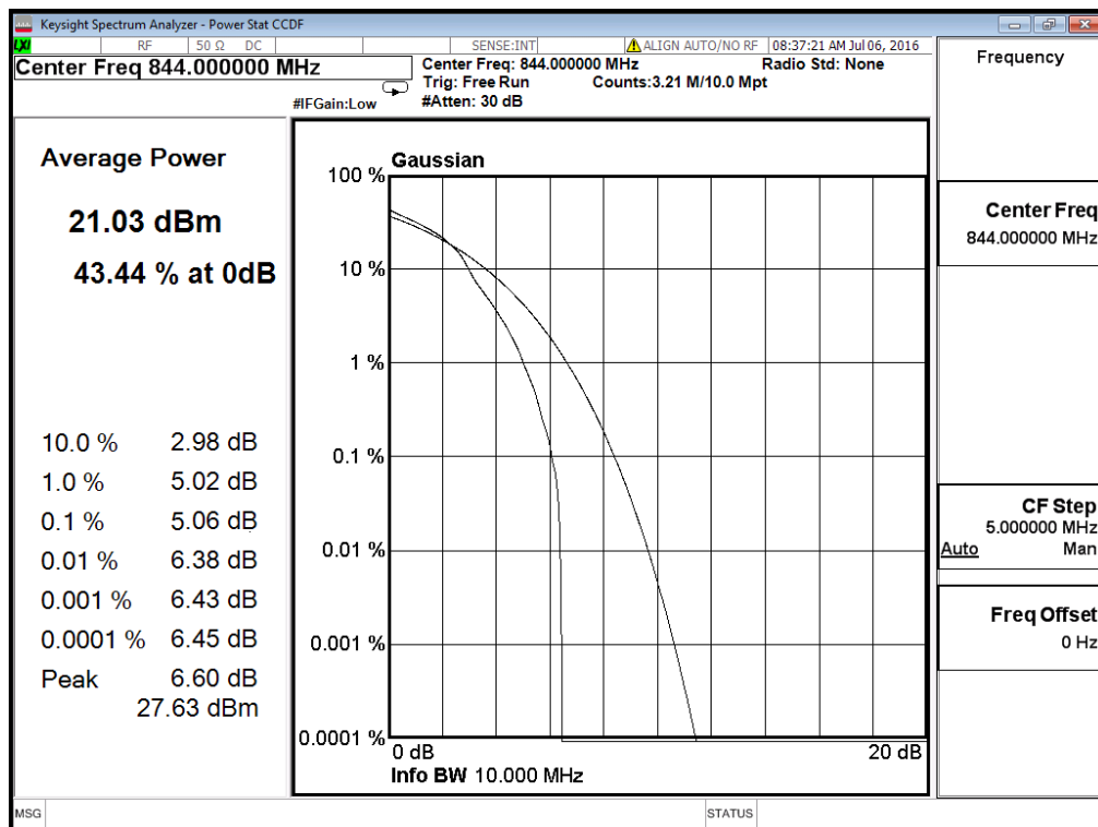
(Plot C5: Band 5/10MHz/16QAM in H Ch 1RB Size)
