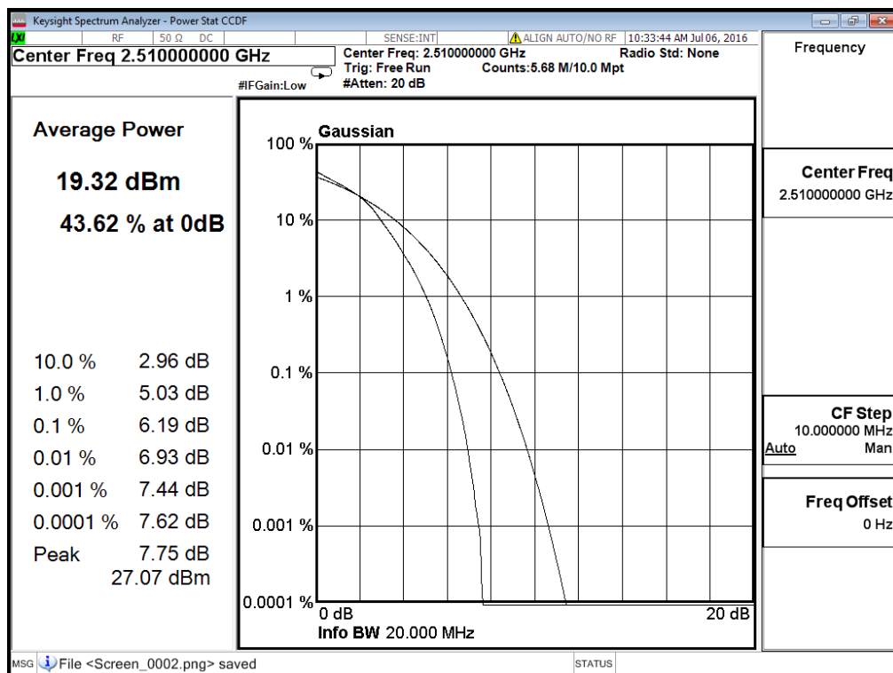
(Plot D2: Band 7/20MHz/16QAM in L Ch 100RB Size)
