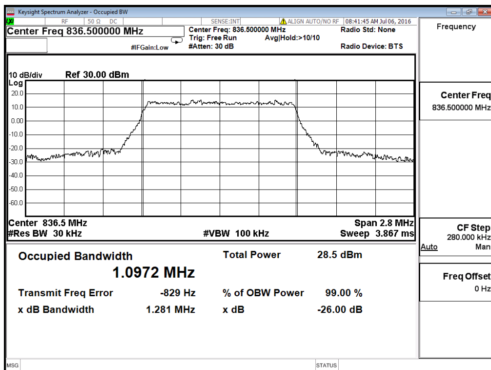
Occupied Bandwidth LTE Band 5/1.4MHz/16QAM
