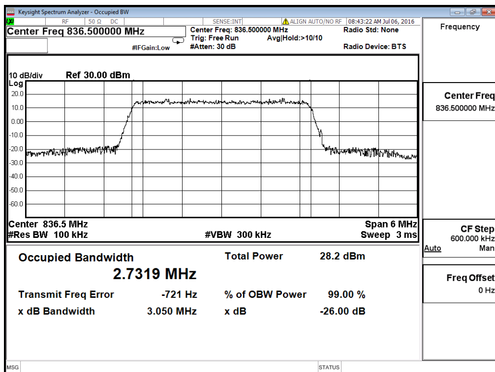
Occupied Bandwidth LTE Band 5/3MHz/16QAM
