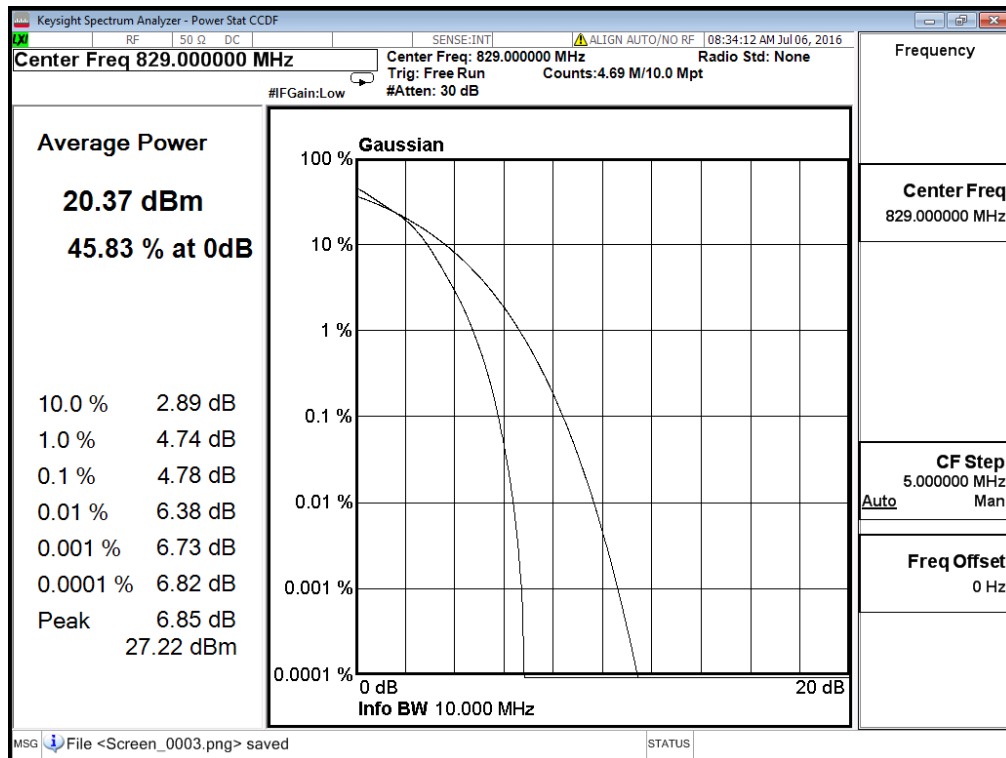
(Plot C1: Band 5/10MHz/16QAM in L Ch 1RB Size )
