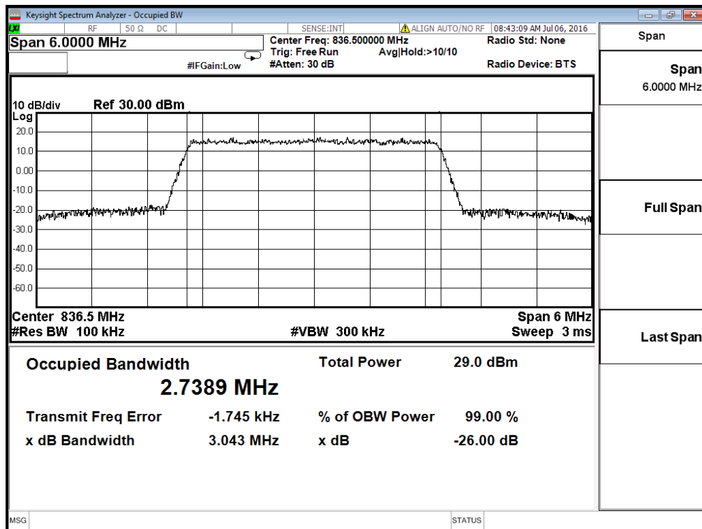
Occupied Bandwidth LTE Band 5/3MHz/QPSK
