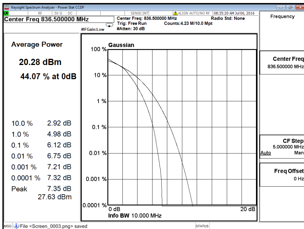
(Plot C4: Band 5/10MHz/16QAM in M Ch 50RB Size)
