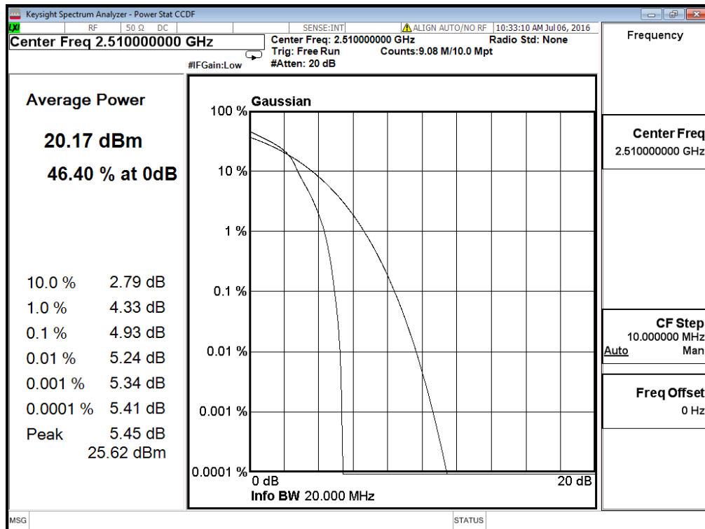
(Plot D1: Band 7/20MHz/16QAM in L Ch 1RB Size )
