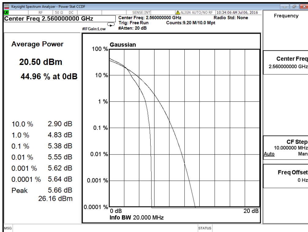
(Plot D5: Band 7/20MHz/16QAM in H Ch 1RB Size)
