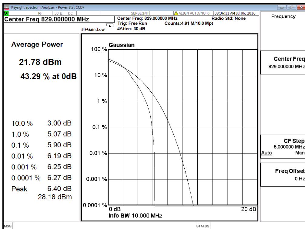
(Plot C2: Band 5/10MHz/16QAM in L Ch 50RB Size)
