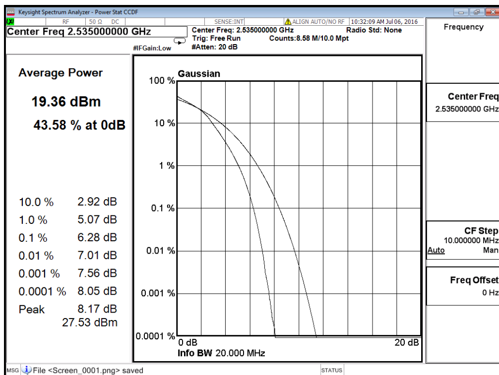
(Plot D4: Band 7/20MHz/16QAM in M Ch 100RB Size)
