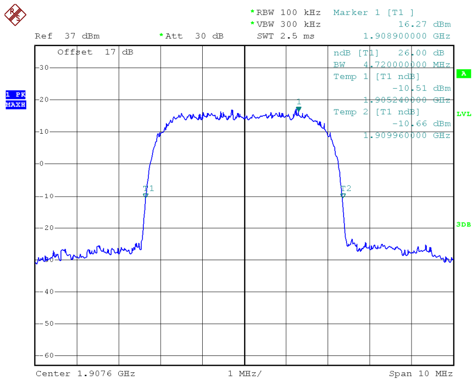
(Plot F3: WCDMA 1900MHz Channel = 9538)
