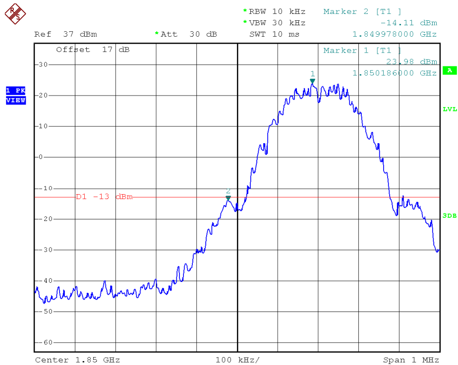
(Plot C: GPRS 1900 Channel = 512)
