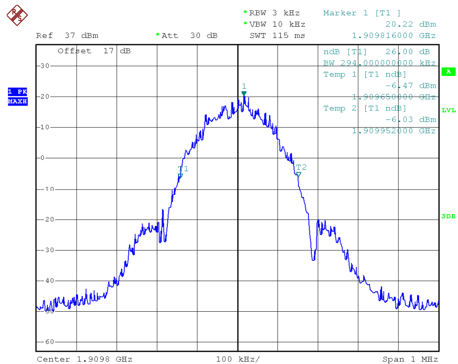
(Plot D3: EDGE 1900MHz Channel = 810)
