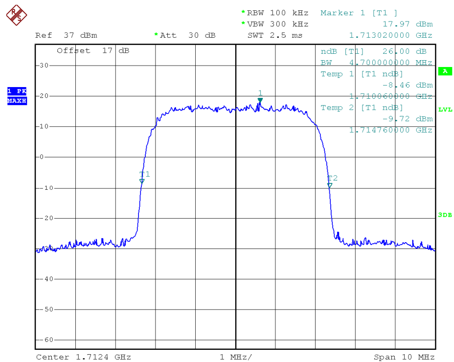
(Plot G1: WCDMA 1700MHz Channel = 1312 bandwidth)
