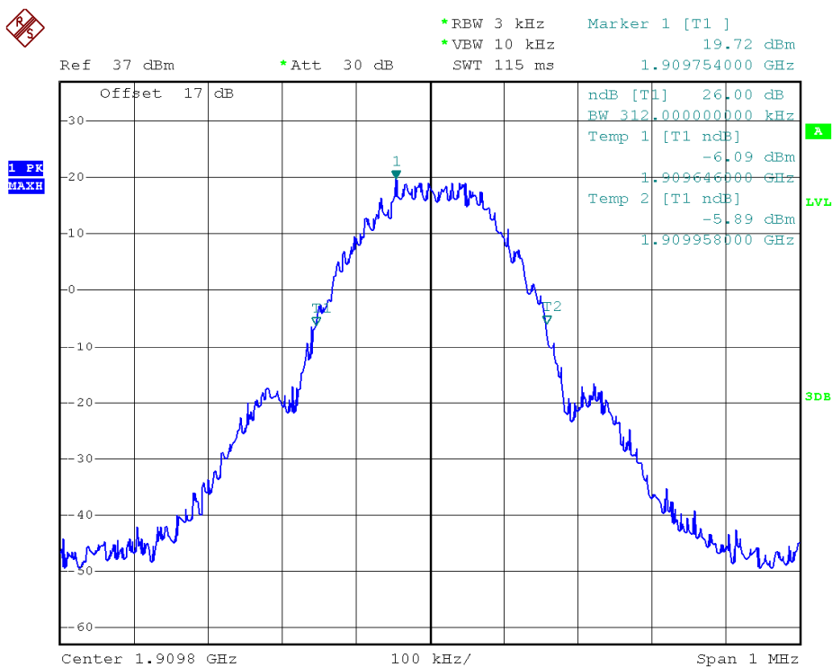
(Plot B3: GPRS 1900MHz Channel = 810)
