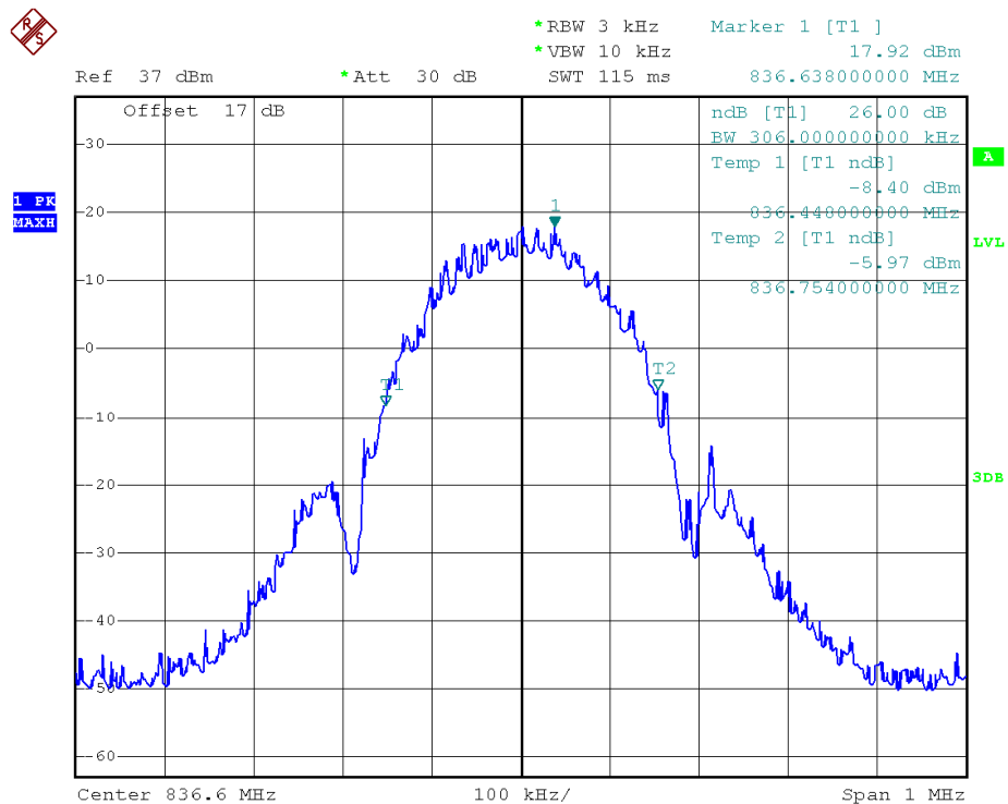
(Plot C2: EDGE 850MHz Channel = 190)
