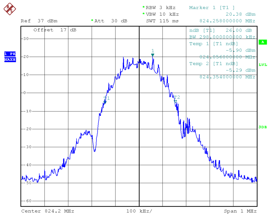
(Plot C1: EDGE 850MHz Channel = 128)
