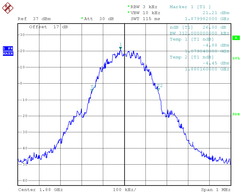
(Plot B2: GPRS 1900MHz Channel = 661)
