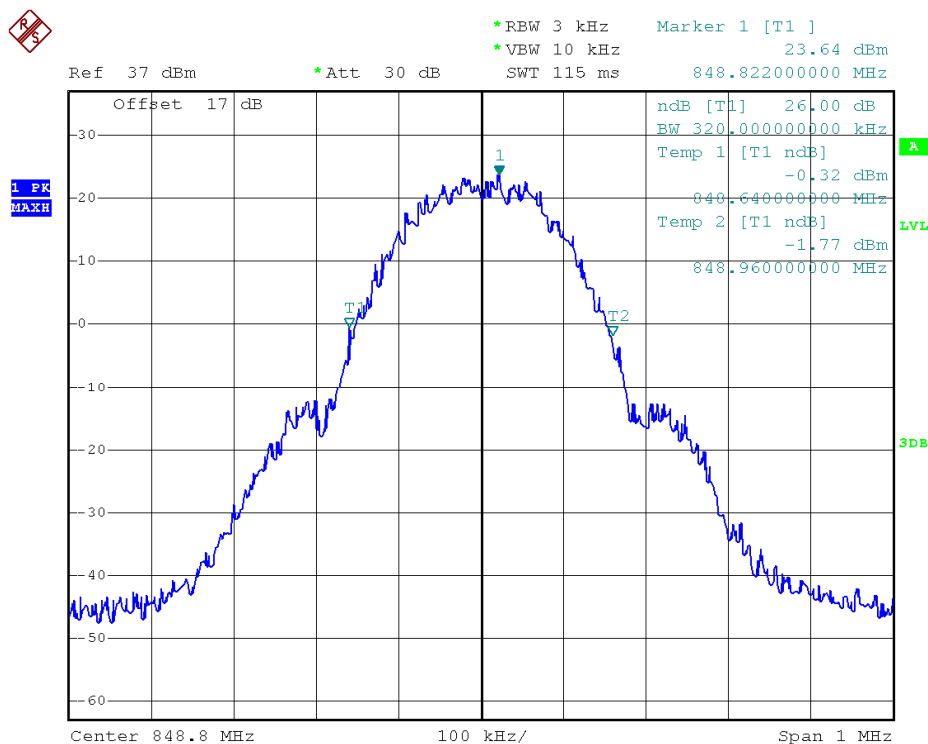
(Plot A3: GPRS 850MHz Channel = 251)
