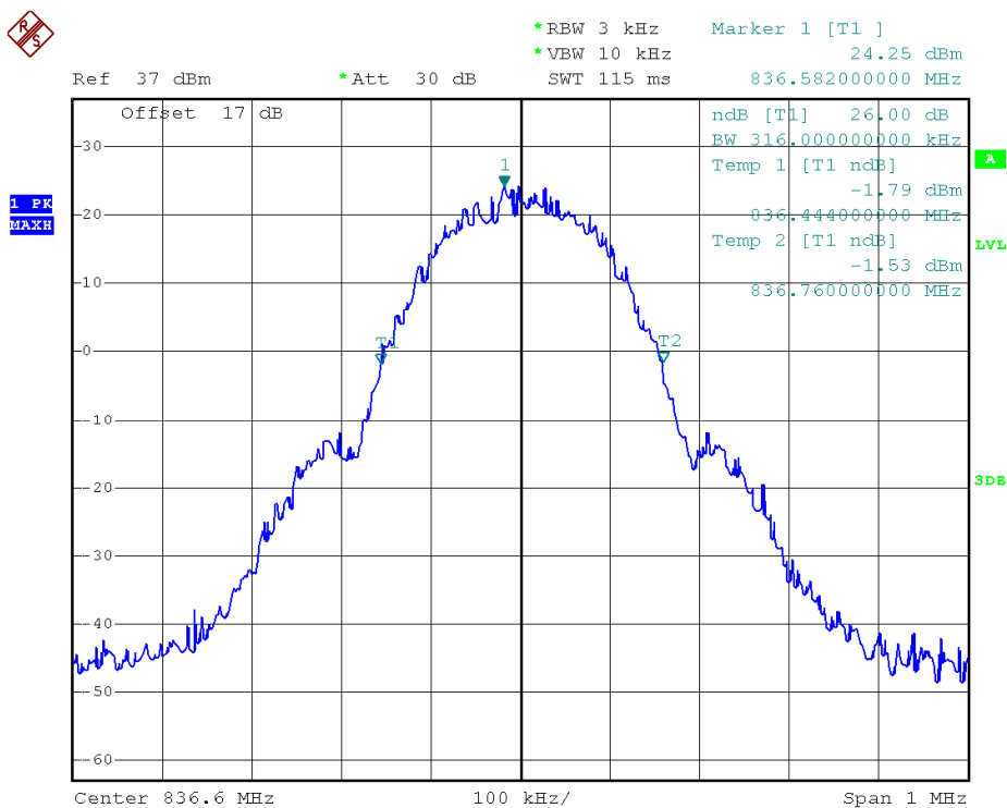
(Plot A2: GPRS 850MHz Channel = 190)
