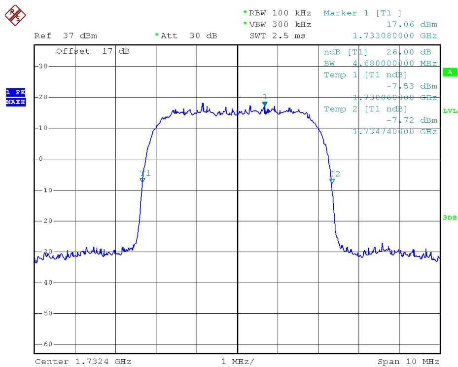
(Plot G2: WCDMA 1700 MHz Channel = 1412 bandwidth)
