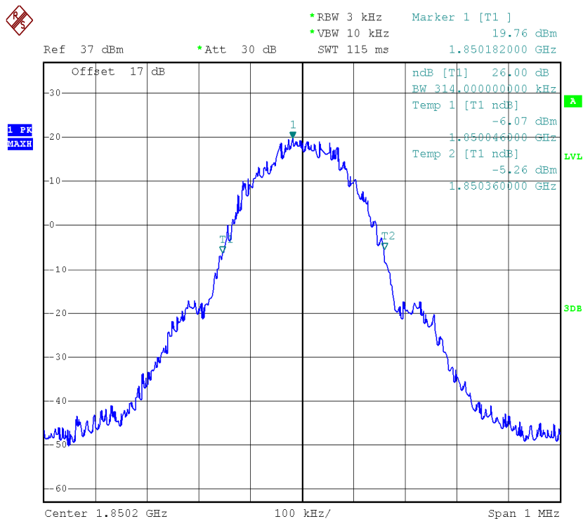
(Plot B1: GPRS 1900MHz Channel = 512)
