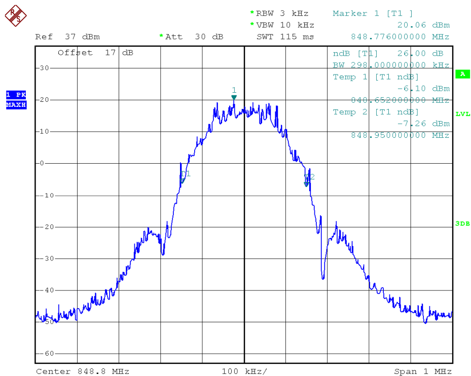
(Plot C3: EDGE 850MHz Channel = 251)
