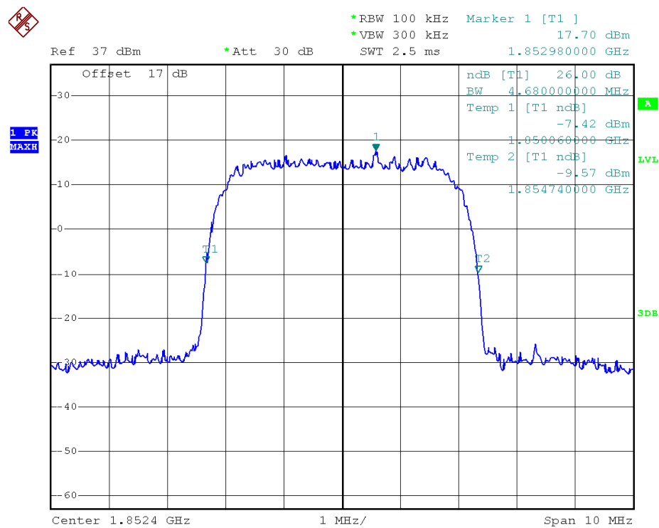
(Plot F1: WCDMA 1900MHz Channel = 9262)
