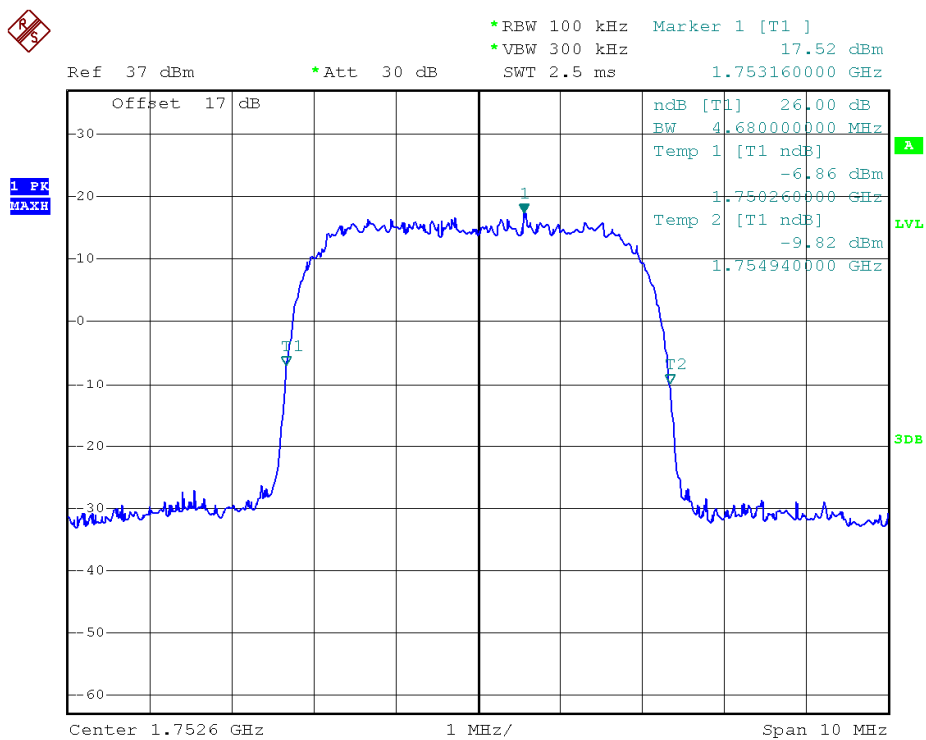
(Plot G2: WCDMA 1700 MHz Channel = 1513 bandwidth)
