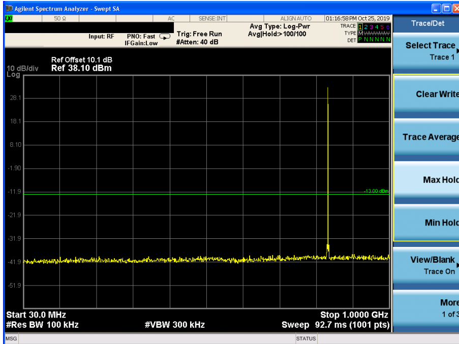
Channel 189, 30MHz~1GHz
