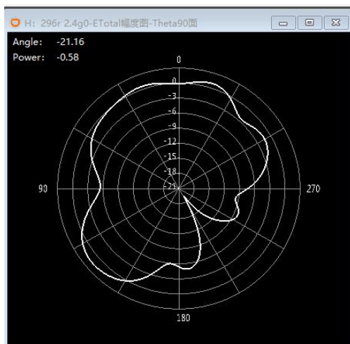
2.4G Wifi 1 antenna
