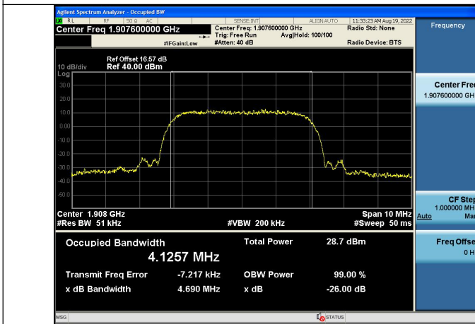
Channel 9538
