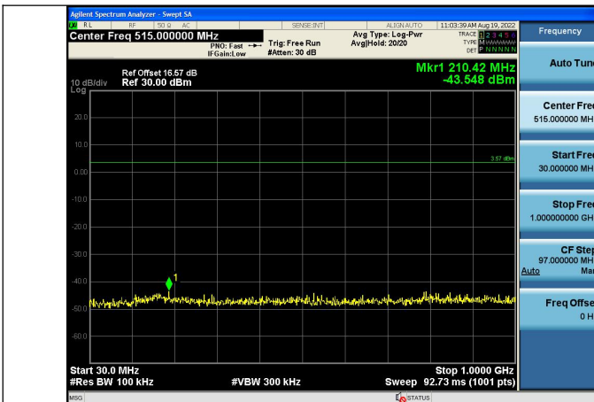
Channel 9262 30MHz~1GHz(dBm)
