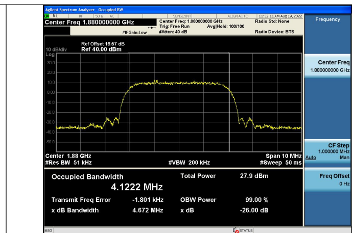
Channel 9400
