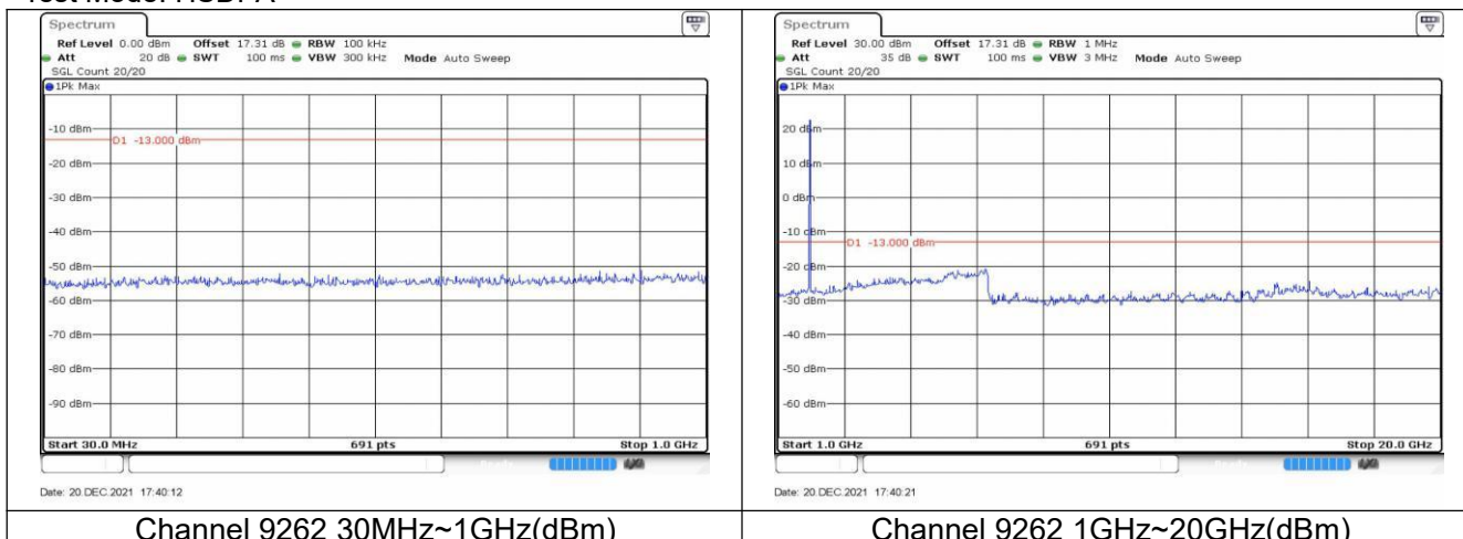
Channel 9262 30MHz~1GHz(dBm)
