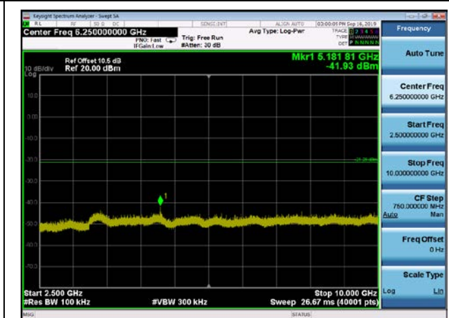
,Plot 4,2500MHz~10000MHz-802.11n(HT40 ) ,2452MHz,Ant1
