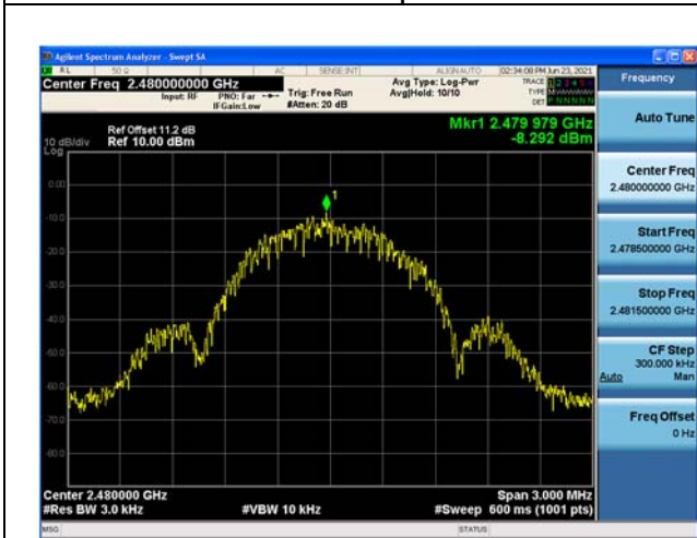
Modulation: 1Mbps 2480MHz
