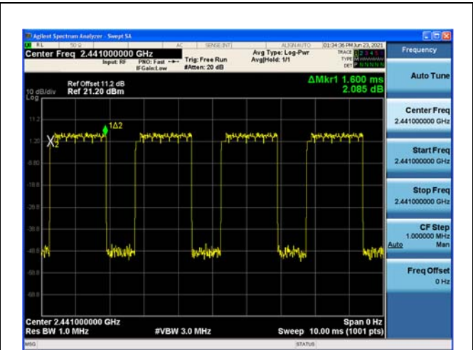
Modulation: 8DPSK DH3 2441
