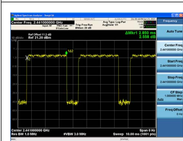
Modulation: 8DPSK DH5 2441
