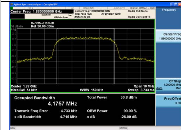
HSDPA Mode: Mid Channel
