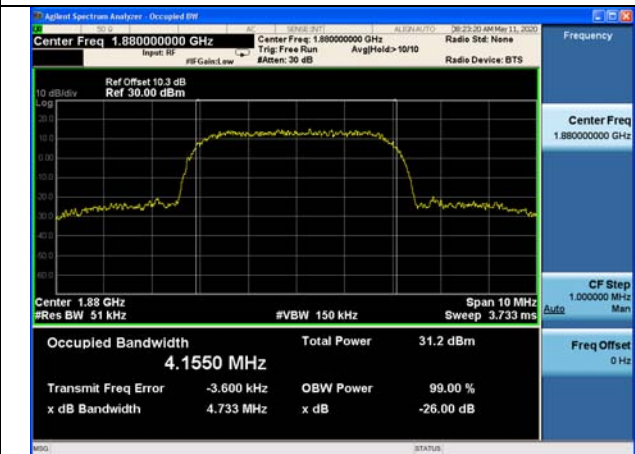
HSDPA Mode: Low Channel
