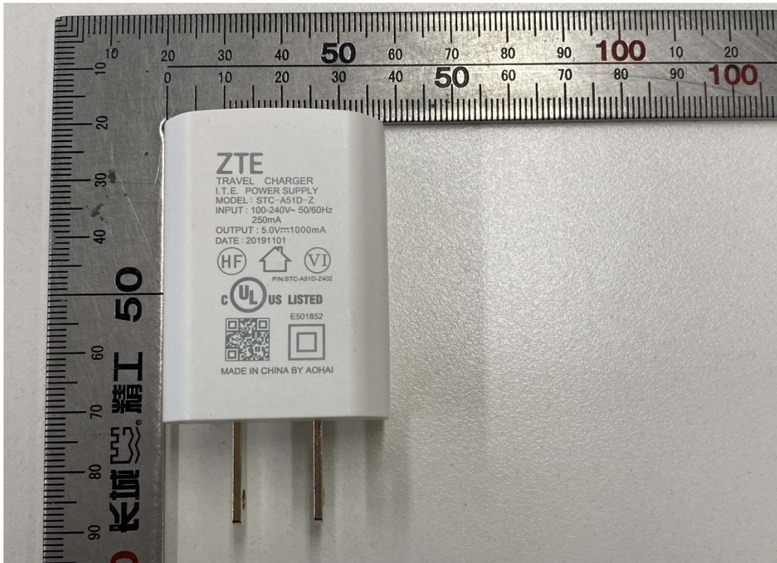
Charger View (Model: STC-A51D-Z made by AOHAI)
