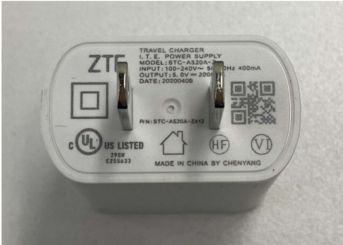
Charger View (Model: STC-A520A-Z made by Chenyang)
