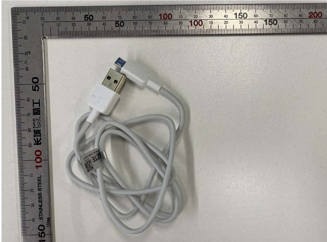
USB Cable made by Shen Zhen Shi Yi HUA XING Electron Co.,Ltd (Model number: USB-MU5-W-100-M)
