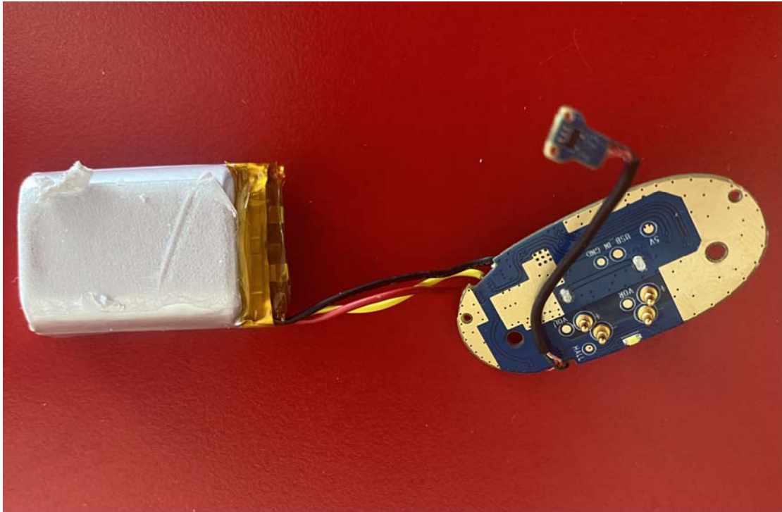
Charger internal photos
