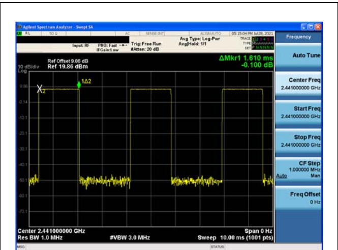
Modulation: GFSK DH3 2441
