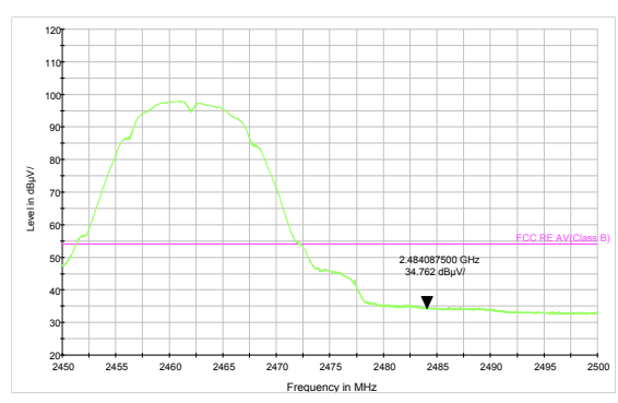
802.11g-Channel 11: Peak
