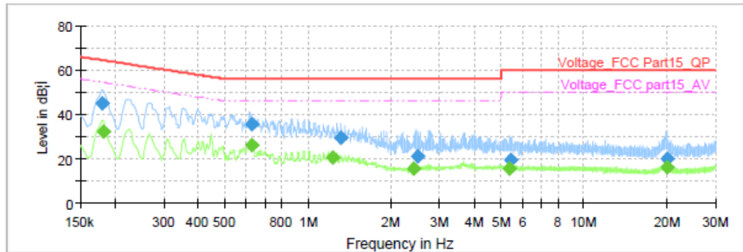
WIFI 2.4G_L_0.15-30MHz
