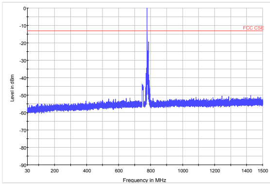
LTE Band 13 10MHz CH- High 30MHz~1.5GHz
