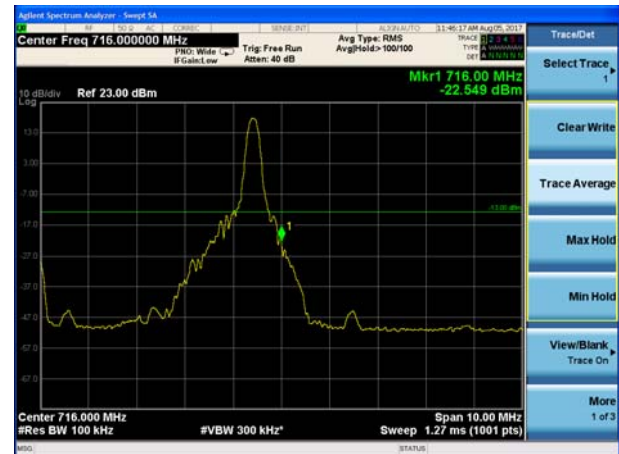
LTE Band 17 16QAM 10MHz CH-High, 1 RB
