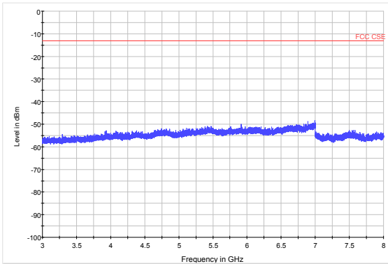
LTE Band 17 5MHz CH-Low 3GHz~8GHz
