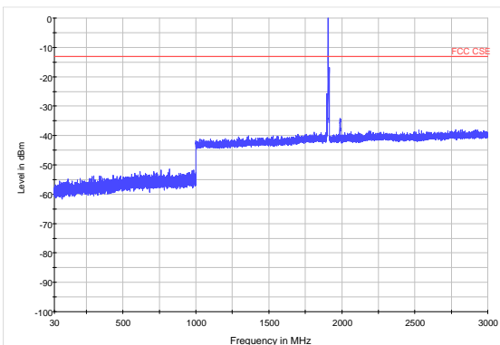
LTE Band 2 5MHz CH-High 30MHz~3GHz
