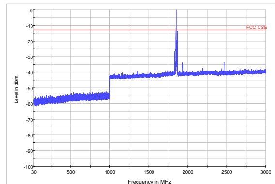
LTE Band 2 10MHz CH-Low 30MHz~3GHz
