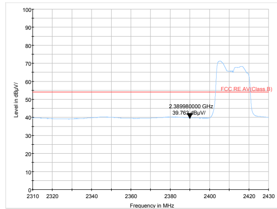
802.11g-Channel 1 Average
