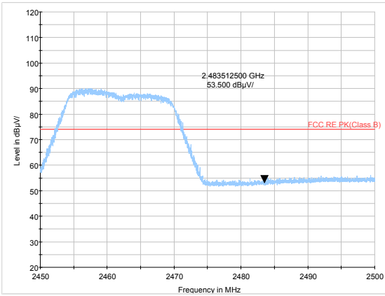
802.11g-Channel 11 Peak
