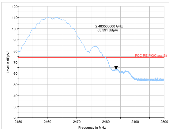
802.11b-Channel 11 Peak
