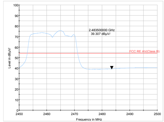
802.11g-Channel 11 Average
