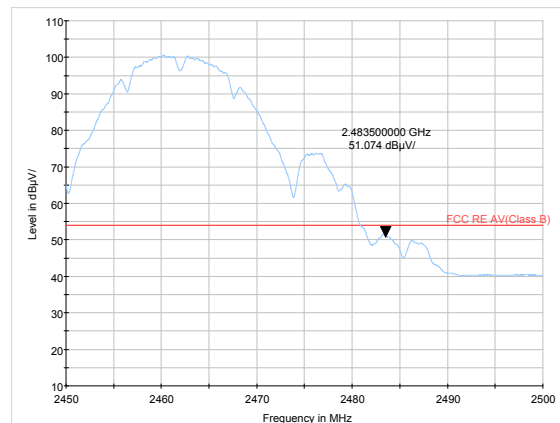
802.11b-Channel 11 Average
