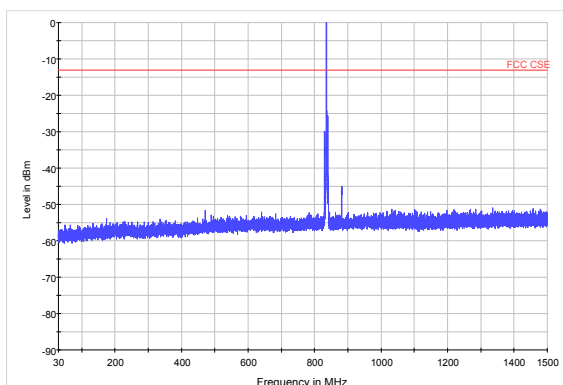
LTE Band 5 3MHz CH-High 30MHz~1.5GHz
