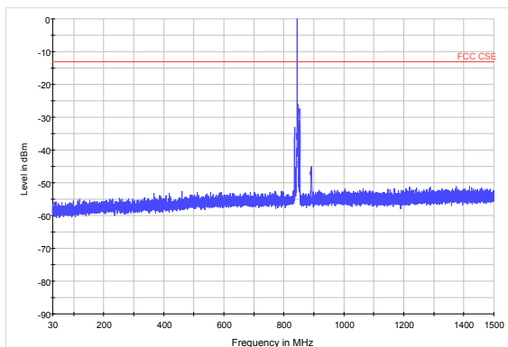
LTE Band 5 5MHz CH-High 30MHz~1.5GHz
