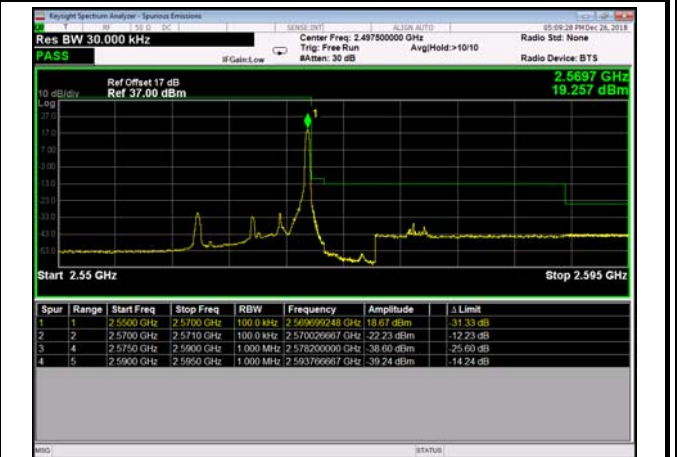
HighRange_FDD07_5MHz_OneRB _high_Q16
