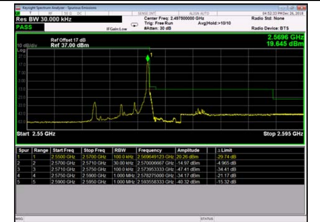
HighRange_FDD07_5MHz_OneRB _high_QPSK
