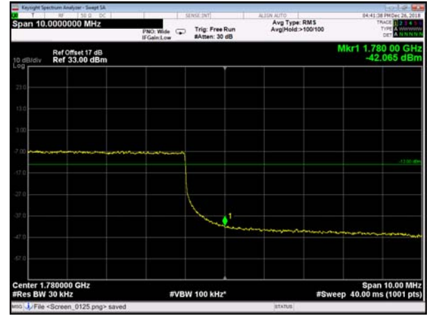
HighRange_FDD66_20MHz_1770_fullIRB _High_Q16
