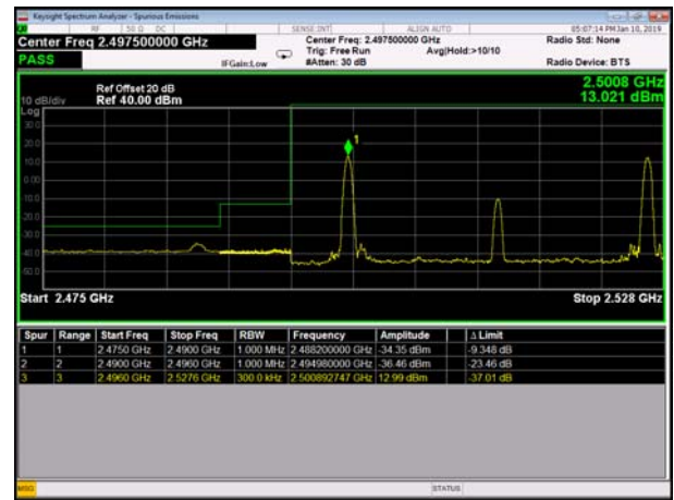
HighRange_FDD07_15+15MHz_1RB0 and 1RB74 Q16
