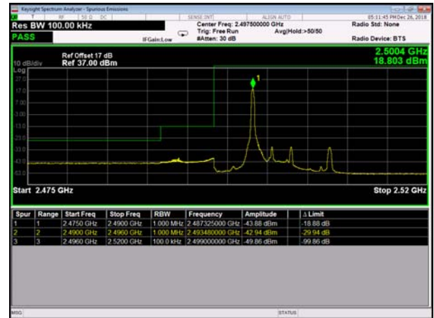
HighRange_FDD07_5MHz_FullIRB _high_Q16
