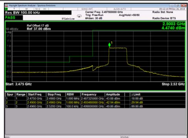
HighRange_FDD07_5MHz_FullIRB _Low_Q16
