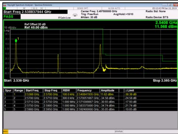
LowRange_FDD07_15+15MHz_FullRB QPSK
