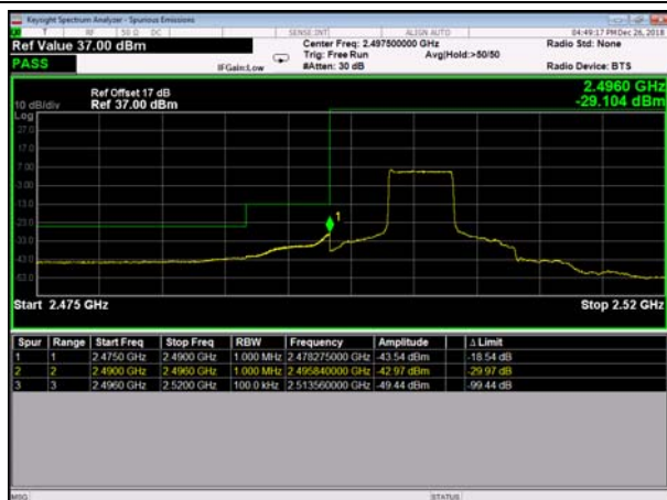
HighRange_FDD07_5MHz_FullIRB _Low_QPSK
