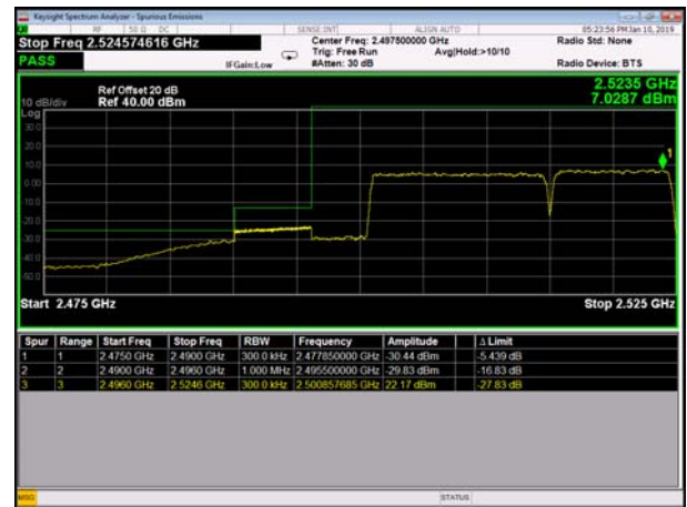
HighRange_FDD07_15+10MHz_FullIRB Q16
