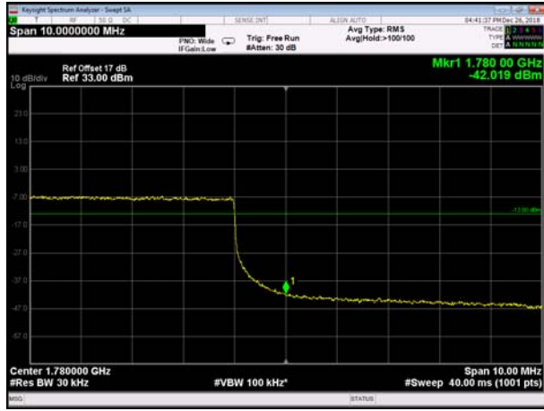
HighRange_FDD66_20MHz_1770_fullIRB _High_QPSK125 126
