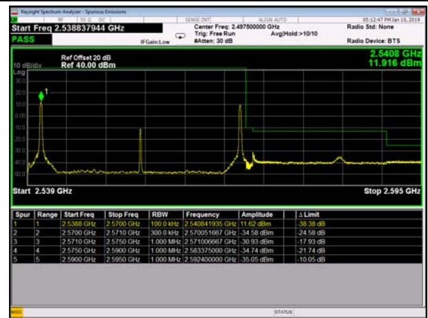
LowRange_FDD07_15+15MHz_FullRB Q16
