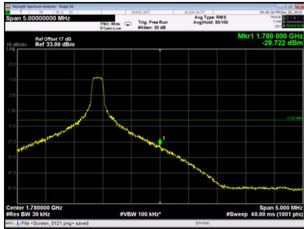
HighRange_FDD66_15MHz_1772.5_fullRB _High_QPSK
