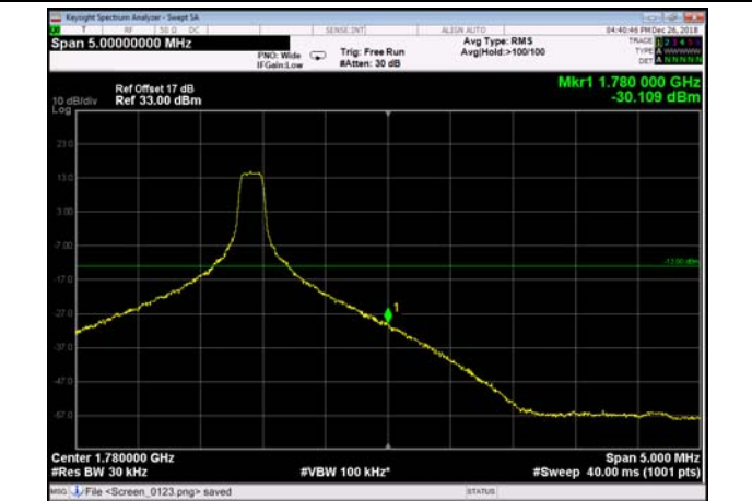
HighRange_FDD66_20MHz_1770_OneRB _high_Q16
