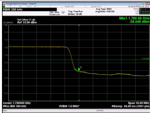
HighRange_FDD66_20MHz_1770_OneRB _high_QPSK
