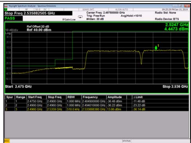
LowRange_FDD07_20+15MHz_FullIRB Q16
