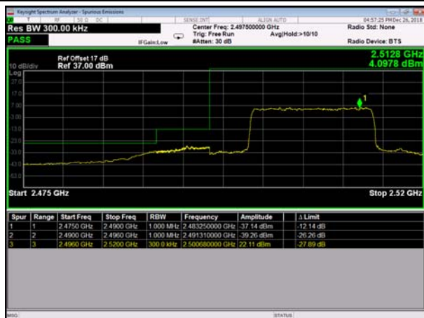
HighRange_FDD07_15MHz_FullRB_Low_QPSK
