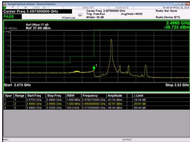
HighRange_FDD07_5MHz_FullIRB _high_QPSK
