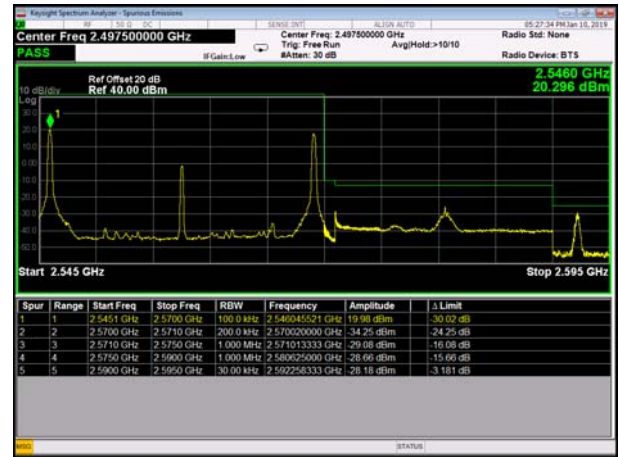
LowRange_FDD07_15+10MHz_FullIRB Q16
