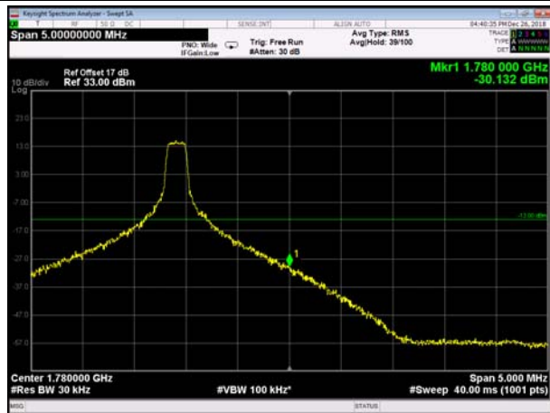
HighRange_ FDD66_10MHz_1775_fullRB _High_QPSK
