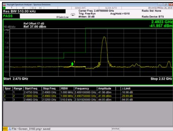
HighRange_FDD07_20MHz_FullRB _high_QPSK
