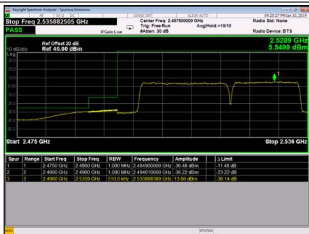
LowRange_FDD07_20+15MHz_FullIRB QPSK
