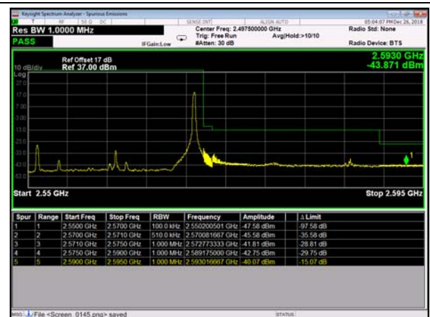
HighRange_FDD07_20MHz_OneRB_high_Q16
