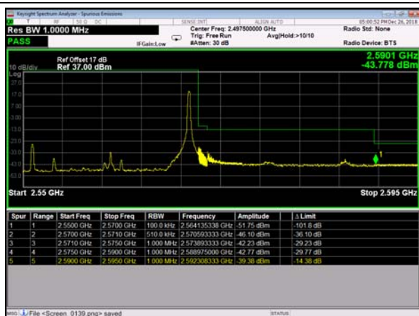
HighRange_FDD07_20MHz_OneRB_high_QPSK
