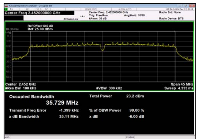
6dB Bandwidth-802.11n(HT40),2452MHz
