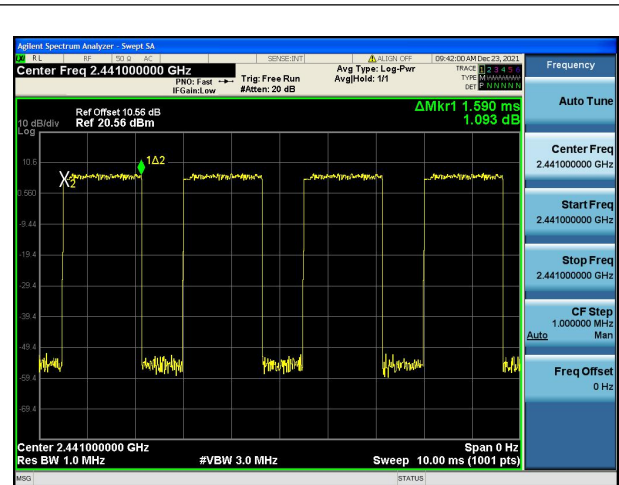
Modulation: 8DPSK 3DH3 2441MHz
