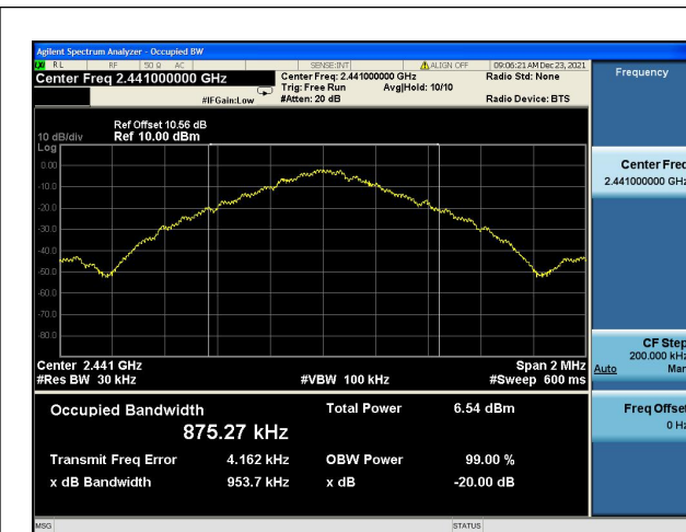
Modulation: GFSK 2441MHz
