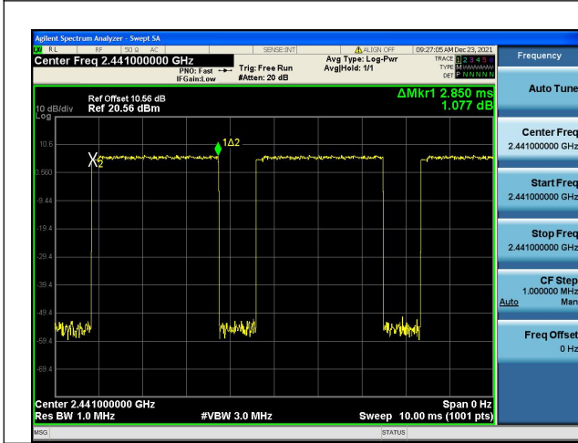
Modulation: \pi/4 DQPSK 2DH5 2441MHz
