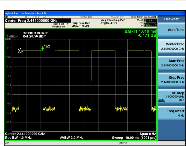
Modulation: GFSK DH3 2441MHz
