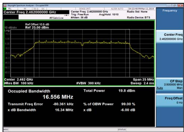
6dB Bandwidth-802.11g,2462MHz
